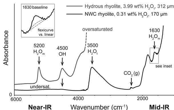
FIGURE 1. \text{H}_2\text{O} absorbance bands in FTIR spectra of hydrous rhyolite glasses. The 5200 and 4500 \text{cm}^{-1} bands can be seen in the thick, water-rich glass (gray spectrum), but the mid-IR bands are oversaturated. In the thinner, water-poor NWC glass (black spectrum, this study), the 5200 \text{cm}^{-1} band is undersaturated and the 4500 \text{cm}^{-1} band is only weakly seen, but the 3500 and 1630 \text{cm}^{-1} bands can be seen. A small doublet can be seen at \sim 2350 \text{cm}^{-1} due to molecular \text{CO}_2 in the atmosphere. Inset compares choice of linear and flexicurve baselines for 1630 \text{cm}^{-1} band.
