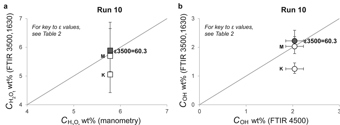
FIGURE 5. FTIR analysis of Fe-bearing andesite standard Run 10. (a) \text{H}_2\text{O}_\text{T} concentration calculated from the 3500 and 1630 \text{cm}^{-1} bands using the species-dependent \epsilon_{3500} method (filled square) is compared to the \text{H}_2\text{O}_\text{T} content measured by manometry. Open squares show \text{H}_2\text{O}_\text{T} calculated using the range of fixed \epsilon_{3500} values for Fe-bearing andesite in the literature (letters indicate source studies for the different \epsilon_{3500} values used, see Table 2 for key to labels). (b) OH concentration calculated from the 3500 and 1630 \text{cm}^{-1} absorbance bands using the species-dependent \epsilon_{3500} method (filled circle) is compared to the OH concentrations calculated from the 4500 \text{cm}^{-1} band via the Beer-Lambert law (Eq. 1). Since the Run 10 sample was too thin to measure the 4500 \text{cm}^{-1} band we use instead the 4500 absorbance reported for this glass in Mandeville et al. (2002). Open circles show OH-by-difference calculated using the range of fixed \epsilon_{3500} values for Fe-bearing andesite in the literature. Solid lines indicate 1:1 lines. Error bars are derived from the \pm 3 \mu\text{m} error on the thickness measurement of this thin sample.
