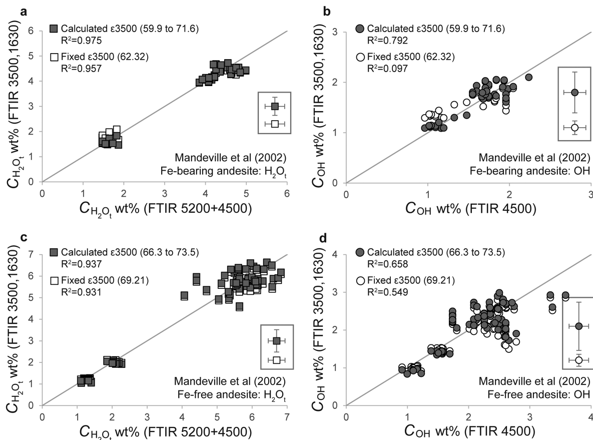
FIGURE 3. Validation of the species-dependent \epsilon_{3500} method for andesite. H 2 O i (squares) and OH (circles) concentrations calculated from the 3500 and 1630 cm -1 bands using the species-dependent \epsilon_{3500} method (filled symbols) are compared to those derived from the 5200 and 4500 cm -1 bands for the published data set of Mandeville et al. (2002) for (a and b) Fe-bearing andesite and (c and d) Fe-free andesite. H 2 O i and OH-by-difference concentrations calculated using the fixed \epsilon_{3500} values of the Mandeville et al. study are shown for comparison (open symbols). Solid line indicates the 1:1 line. For clarity, errors calculated from uncertainties on all values of \epsilon used by each method are shown as symbols with representative error bars on the right-hand margin of each figure tile.
