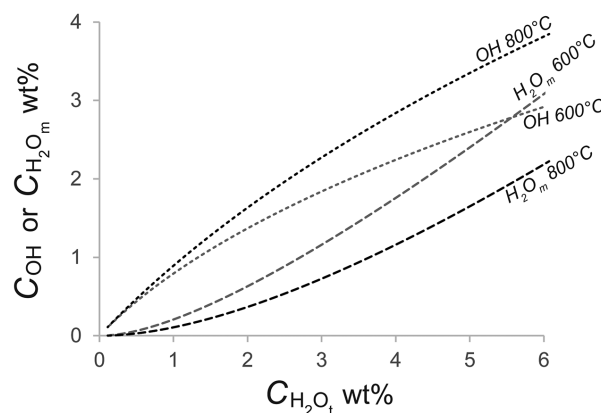
FIGURE 6. Example of experimentally determined water speciation model showing variation in OH and \text{H}_2\text{O}_\text{m} concentration with \text{H}_2\text{O}_\text{i} concentration at different temperatures for haplogranite composition (Nowak and Behrens 2001). OH is the dominant species at low- \text{H}_2\text{O}_\text{i} concentrations and higher temperatures.
