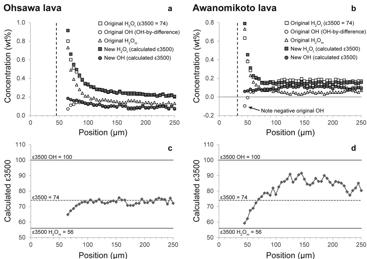
FIGURE 7. Recalculation of the obsidian hydration profiles published by Yokoyama et al. (2008) for (a) Ohsawa and (b) Awanomikoto lavas from Kozushima, Japan. The original profiles (open symbols) were obtained using a fixed value of \epsilon_{3500} = 74 and are shown alongside \text{H}_2\text{O}_\text{t} and OH profiles recalculated using the species-dependent \epsilon_{3500} method (filled symbols). Note the negative OH values in the original Awanomikoto profile (b). The vertical black dashed lines represent the position of the glass edge; profiles are truncated where Yokoyama et al. (2008) calculated that there would be no contamination from the adjacent resin. (c and d) The “true” (species-dependent) \epsilon_{3500} values calculated for each position in the recalculated profiles are shown with reference to the \epsilon_{3500} end-member values for rhyolite and the original choice of fixed \epsilon_{3500} = 74 .
