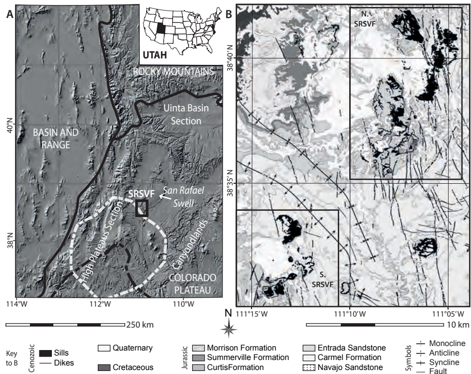
Fig. 1. Location maps for the San Rafael Sub-Volcanic Field in Utah. (A) Digital elevation Model for Utah, showing major structural and depositional areas of the Colorado Plateau. Solid black line shows province boundaries. Dashed black line is a region of lower-crustal delamination and crustal thinning detailed in Levander et al. (2011); dashed white line is their outline of a downwelling body at 200 km depth, estimated from body wave tomography. (B) Geological map of the region of interest, showing relative positions of the Northern (N.) and Southern (S.) SRSVF.
