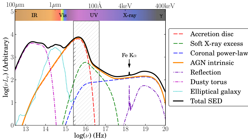
Figure 1. A simplified schematic diagram of an AGN SED, showing the approximate shape and extent of the various components discussed in the text. Dashed lines denote AGN intrinsic emission, dash-dotted lines show emission reprocessed by the surrounding material and the dotted line shows starlight from an elliptical host galaxy. The hatched region highlights the spectral range that is heavily obscured by absorption in the IGM. We only show an elliptical galaxy here; galaxies with active star formation have stronger UV/IR contributions.
