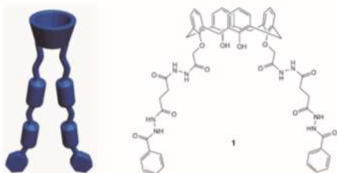
Scheme 1. Structure of gelator 1 and schematic representation
