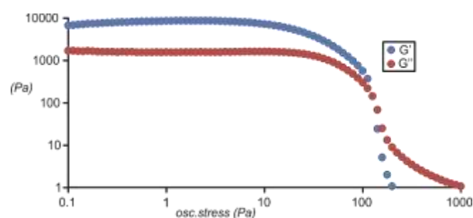
Figure 2 stress sweep rheometry for a 2% w/v gel of 1 in 1,2-dibromoethane.
