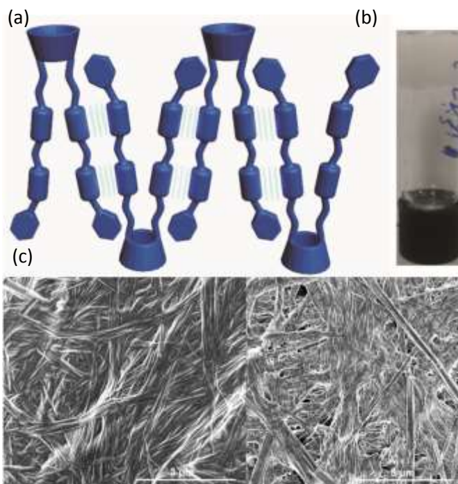
Figure 1 (a) schematic of the proposed self-assembly of 1 to produce a gel fibre (b) vial inversion test of the 1,2-dibromoethane gel of 1 (2 % w/v) (c) SEM images of the xerogel.
