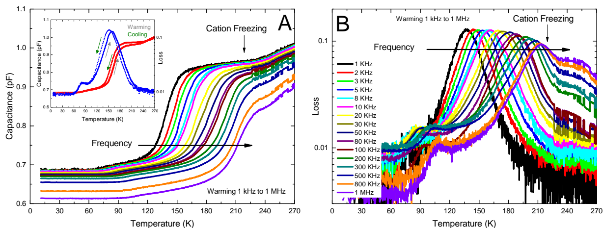
Fig. 2 Capacitance (A) and loss (B) data for TEA(TCNQ) 2 showing anomalies at ~220 K and ~100 K. Inset : Warming and cooling data for the capacitance and loss at 10 kHz, the green arrows and grey arrows correspond to the cooling and warming curves respectively.
