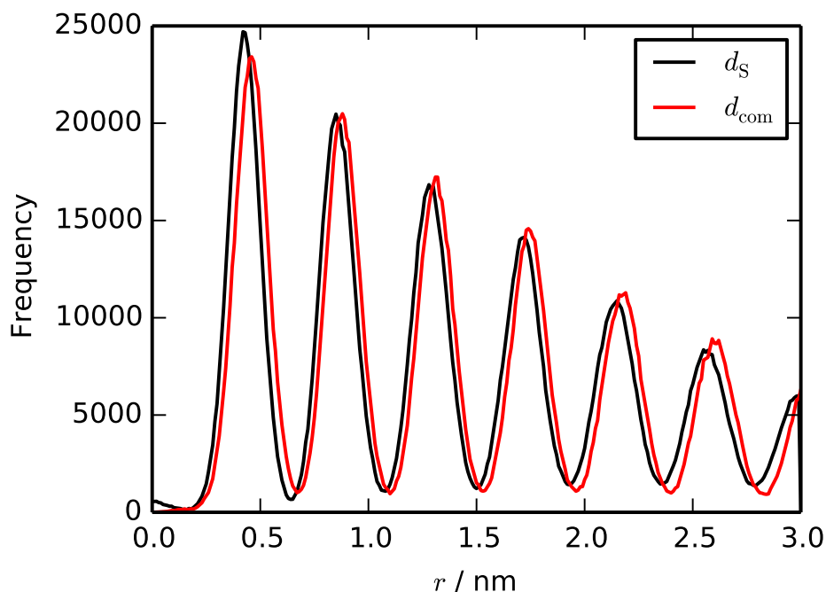
Figure 3. Probability distributions for the pair distances, d_{\text{com}} , and d_S for a single chromonic stack simulated at 280 K using the MARTINI model for TP6EO2M.
