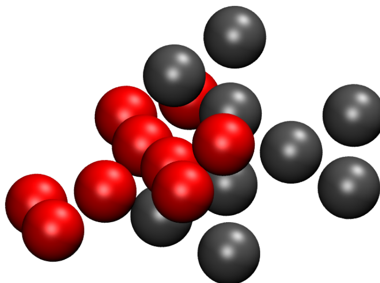
Figure 6. Simulation snapshot of a dimer using the original SAFT model with unadjusted bond lengths, with the core-core distance constrained at 0.55 nm. Only the aromatic cores are shown.
