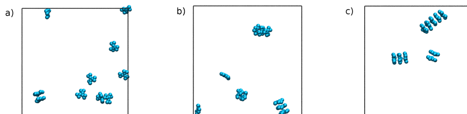
Figure 2. A series of snapshots taken from the simulation of the MARTINI model of TP6EO2M in water at 280 K, showing the central aromatic core of molecules, taken at a) the start of the simulation, b) 50 ns and c) 90 ns. The simulation trajectory shows the spontaneous self-assembly of short chromonic stacks.
