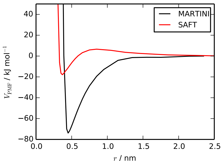
Figure 4. Potential of mean force curves calculated for the separation of a dimer of two molecules for the MARTINI model and the SAFT- \gamma model.
