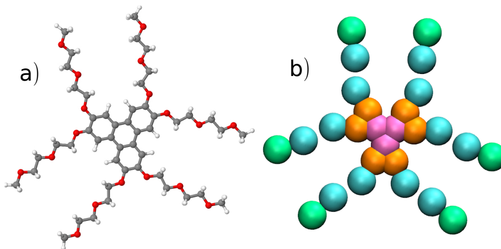
Figure 1. a) Molecular structure of the chromonic liquid crystal, TP6EO2M. b) Coarse-grained mapping used in this work, showing four bead types: CC - pink, CO - orange, AI - blue, AO - green.
