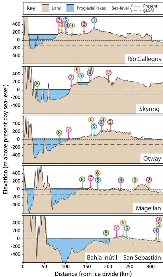
Figure 14. Topographic profiles for each ice lobe, shown as changes in elevation relating to present-day sea-level against distance from the hypothesized ice sheet divide. Ice flowed from left to right. The profiles from the ice divide to the outermost time step are shown in Fig. 13A and B. The coloured numbers relate to the time steps shown in Fig. 13D. Present-day sea-level is shown (short dashes), as well as the approximate sea-level at the gLGM (long dashes). Hence, the outermost limits of the BI-SSb lobe were in the Atlantic Ocean but would have formed on the exposed continental shelf. Also shown are the approximate heights of former proglacial lakes. The Río Gallegos lake would have dropped progressively over time, but the timing is not well constrained.
