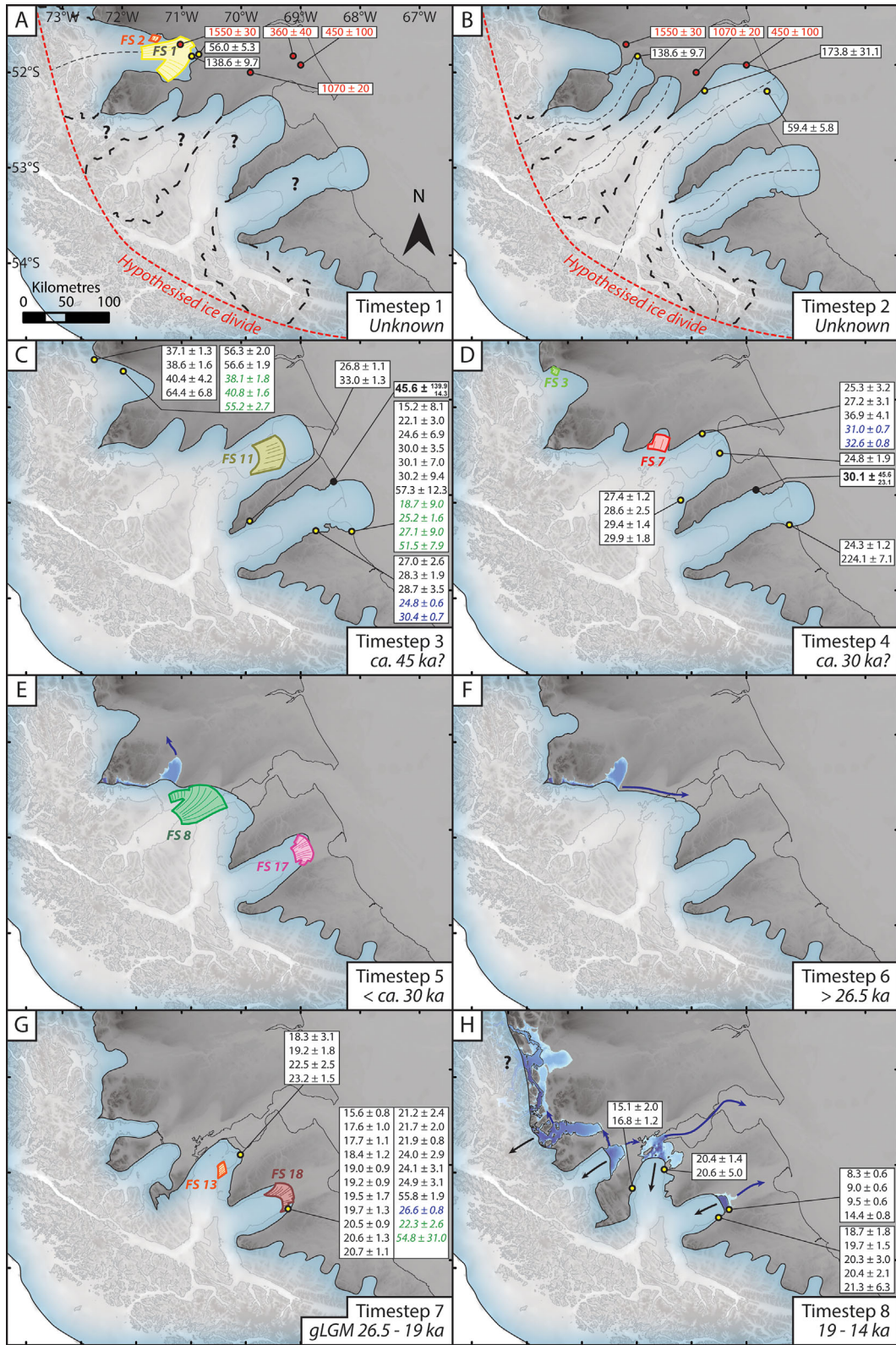
Figure 13. Reconstructed glacial history for the five ice lobes studied, with eight time steps shown in (A) to (H). The hypothesized ice divide based on Hulton et al. (2002) is shown in (A) and (B) for reference. We show the rest of the ice sheet for completeness, with hypothesized gLGM limits based on Coronato et al. (2004). The rest of the ice sheet would have retreated over time, but that was not part of our study. Also shown in (A) and (B) are hypothesized drainage divides between the five ice lobes (bold dashed black lines) and the lines of topographic profiles for each ice lobe shown in Fig. 14 (fine dashed black lines). Key flow-sets are shown and blue arrows show the direction of lake drainage routes. Question marks show where the ice configuration is unknown and black arrows in (H) show final retreat during time step 8. Published chronological data are shown where appropriate (see text for discussion). These are: argon dates (red text/circles); cosmogenic nuclide exposure dates (yellow circles) consisting of recalibrated ^{10}\text{Be} dates (black text), recalibrated ^{26}\text{Al} dates (italic blue text) and ^{36}\text{Cl} dates (italic green text); and cosmogenic nuclide depth profiles (bold black text/circles).
