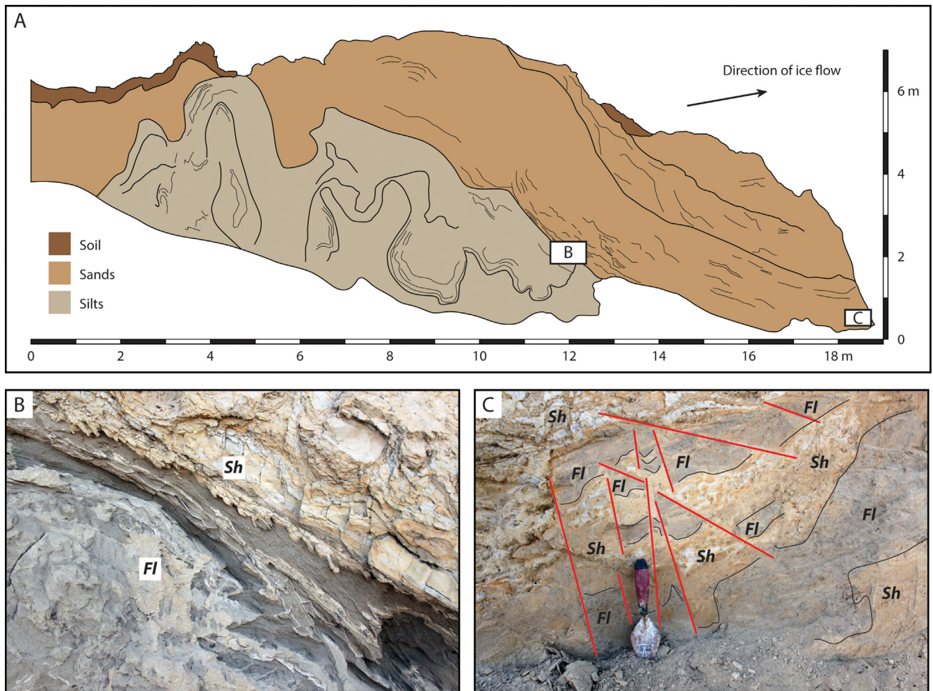
Figure 5. Sketch log (A) and accompanying photographs (B,C) of proglacially tectonized lacustrine silts and sands within an end moraine of the BI-SSb lobe (location shown in Fig. 3A). There is a high degree of folding and faulting. The large section suggests that the ice lobe retreated sufficiently for a sizeable proglacial lake to develop, before re-advance.
