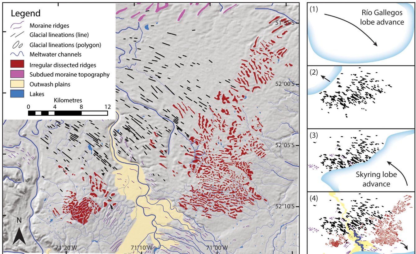
Figure 9. Glacial geomorphology found at the intersection between the Río Gallegos and Skyring lobes (location shown in Fig. 2). (1) to (4) show a stylized formation mechanism for the irregular dissected ridge features. (1) The Río Gallegos advances first, creating a swathe of drumlins (2), and possibly moraines, that are later overridden by an advance of the Skyring lobe (3). The order is dictated by the flow of meltwater from the Skyring lobe into the Río Gallegos basin (4).
