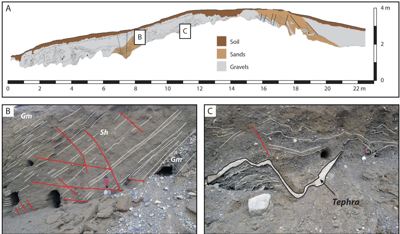
Figure 6. Sketch log (A) and accompanying photographs (B,C) of a glaciotectionized moraine associated with re-advance of the Otway lobe (location shown in Fig. 2). The normal thrust faults are particularly highlighted by a deformed tephra layer in (C). The sediments are characteristic of outwash material that was probably deposited during retreat of the ice before re-advance and proglacial thrusting.
