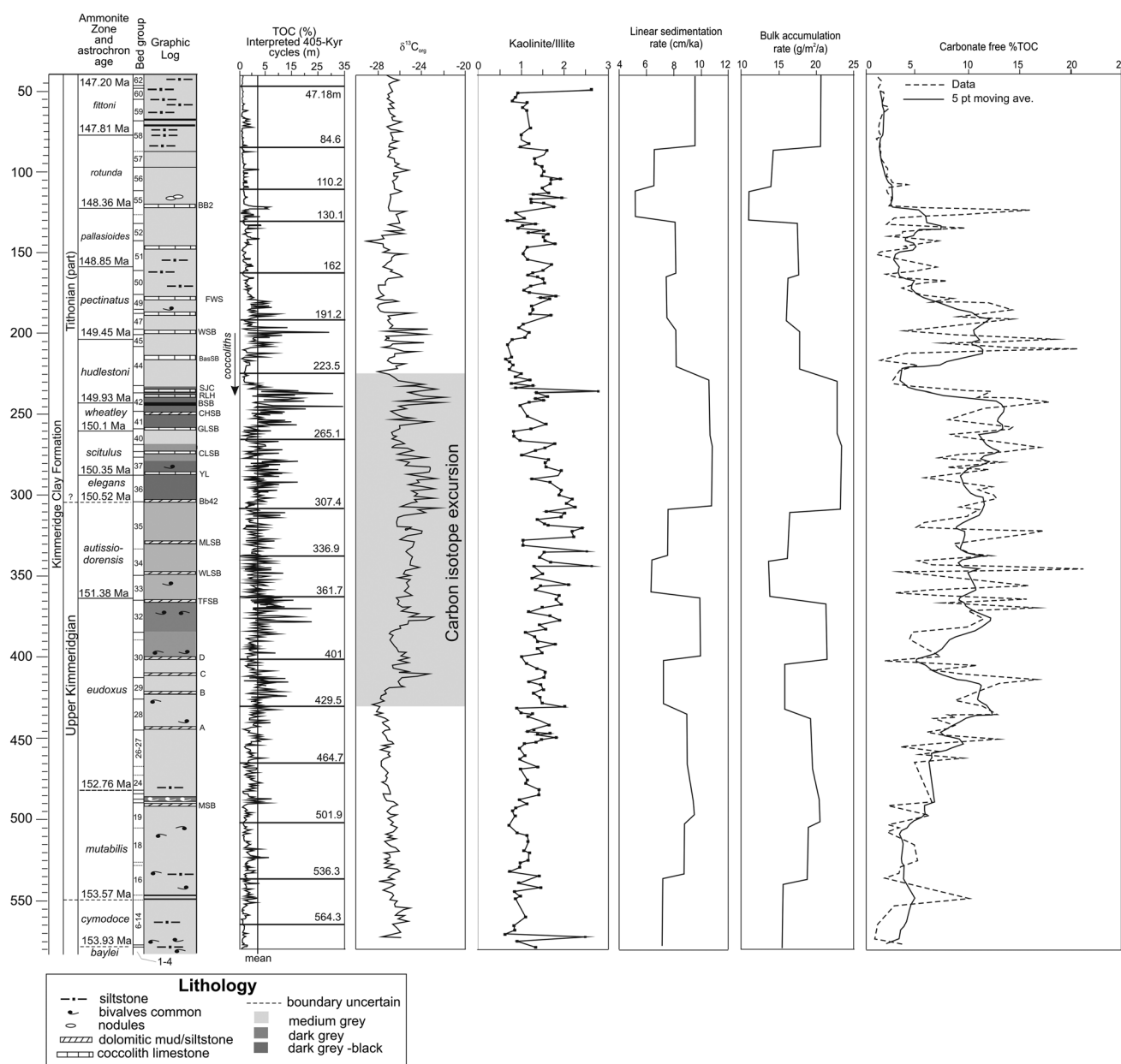
Figure 4. Conflated records of key sedimentological, climate and organic carbon burial proxy data from the Kimmeridge Clay Formation in Dorset. Chronostratigraphy, lithostratigraphy, \delta^{13}\text{C}_{\text{org}} , %TOC are after Morgans-Bell et al. [2001]; clay mineral data are from Hesselbo et al. [2009]. Stone Bands: BB2, Blake's Bed 2; FWS, Fresh Water Steps; WSB, White Stone Band; BaSB, Basalt; SJC, Short Joint Coal; RLH, Rope Lake head; BSB, Blackstone Band; CHSB, Clavell's Hard; GLSB, Grey Ledge; CLSB, Cattle Ledge; YL, Yellow Ledge; Bb42, Blake's Bed 42; MLSB, Maple Ledge; WLSB, Washing Ledge; TFSB, The Flats; MSB, Metherhills.
