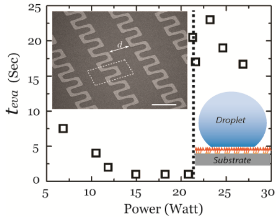
Electro-thermally activated Leidenfrost levitation upon selectively heated substrate
