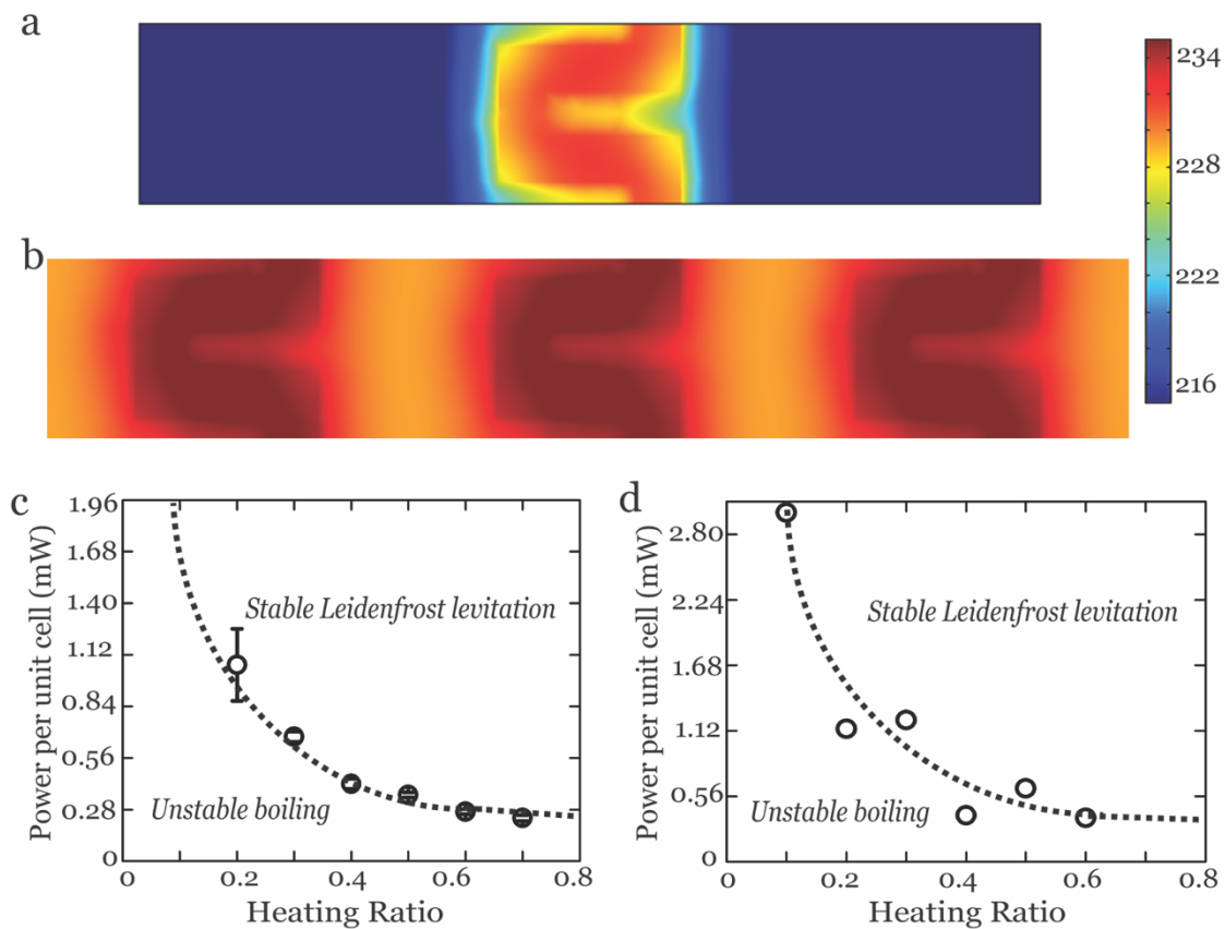
Figure 3. Selective Leidenfrost mechanism and phase diagrams. (a) Temperature profile of surface for the electro-heating of single unit cell with a 0.2 heated ratio. The COMSOL simulation in (b) reveals a uniform distribution of the temperature (in degrees Celsius) across the unit cells within three adjacent serpentine units (a heated ratio of 0.5). The simulation is based on 363 serpentine unit cells in series, which are referred to as a line, and a number of these lines are connected in parallel to form a complete heating array. The applied voltage is then varied to provide an equivalent power per cell required for the Leidenfrost effect to occur. The selective Leidenfrost effect using this pattern is described by phase diagrams on (c) a glass substrate and (d) a silicon substrate. The dotted lines represent the simulation results and the symbols represent the experimental results, respectively.
