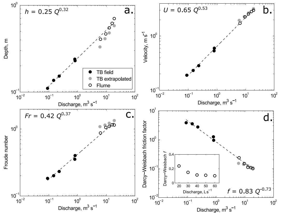
Figure 2. Comparison of calculated reach-averaged (a) depth ( h ), (b) velocity ( U ), (c) Froude number ( Fr ), and (d) Darcy-Weisbach friction factor ( f ) from the field site Trout Beck and from these flume experiments. Flume data are scaled to field dimensions. Two sets of field data are presented. TB field are data collected during low flow conditions using salt dilution gauging. Field data from higher discharges are unavailable due to the difficulty of measuring in high flow. TB extrapolated are values extrapolated from the low flow conditions to higher discharges. Flume data are from the range of discharges used in this study; data from lower discharges are unavailable due to the difficulty of measuring very shallow flows. Flume flow depths are the average from the 18 positions where ADV data were collected. Average velocity is calculated from the bulk discharge and this average flow depth. Dashed lines show power law regressions to the flume and TB field data. All regression R^2 values are > 0.99 , and 95% confidence intervals on all coefficients and exponents show that they are significantly different to zero. Inset in Figure 2d shows just the relationship for flume data using the original flume dimensions.
