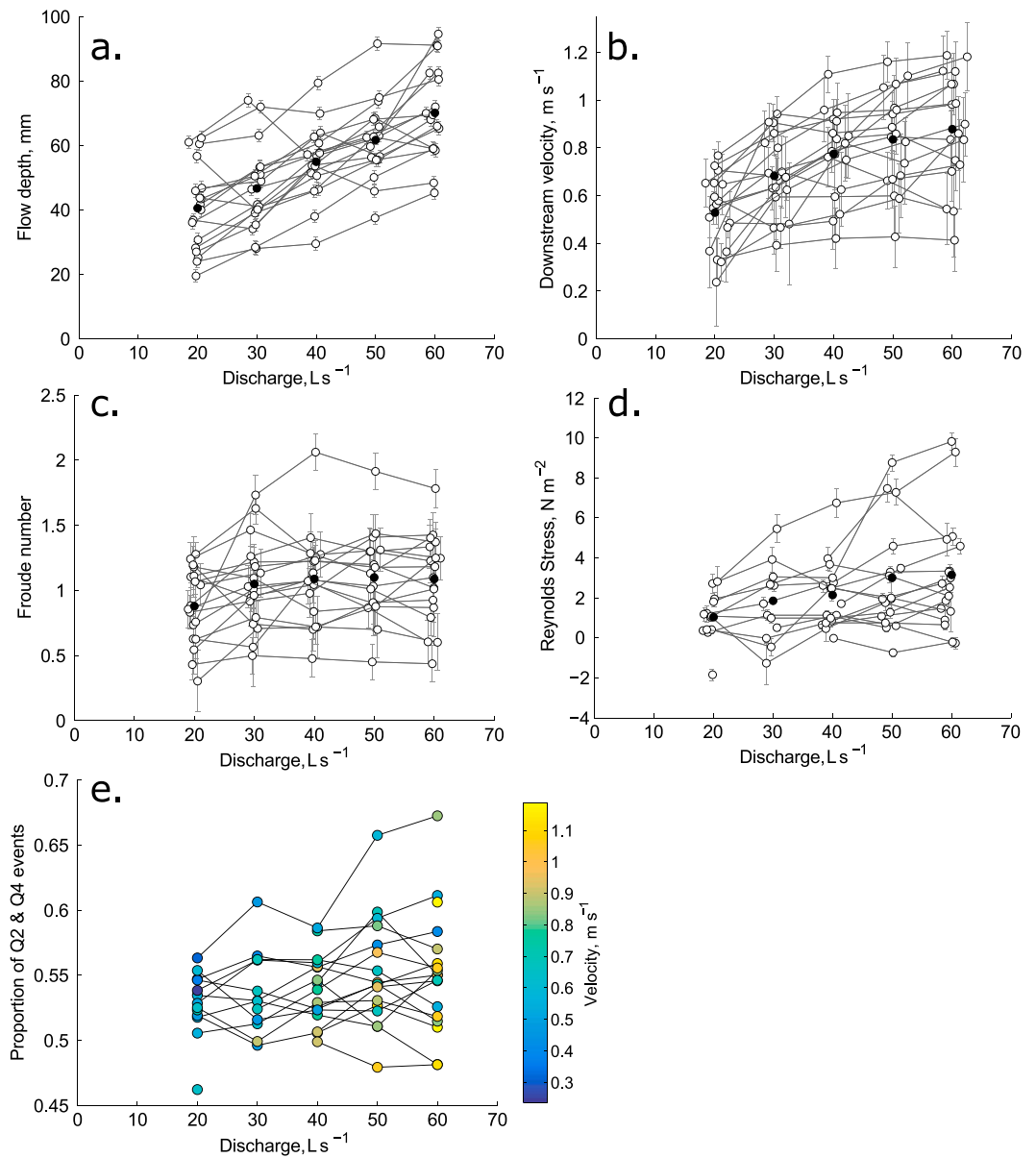
Figure 3. Increase in (a) flow depth, (b) downstream velocity, (c) point Froude number, and (d) point Reynolds stress with increasing discharge in clear water runs. In Figure 3a black points are the mean flow depth. Measurement errors are \pm 2 mm. In Figure 3b velocity is measured at an elevation of 15 mm for most locations. Black points are the mean downstream velocity. Error bars are 1 standard deviation of the ADV measured velocities; error bars of 1 standard error of the mean plot within the circular markers. In Figure 3c black dots are average Froude numbers. Error bars are calculated using \pm 1 standard deviation of the velocity measurements. In Figure 3d black dots are average Reynolds stresses. Error bars are 1 standard error of the mean. (e) The proportion of turbulent flow events in quadrants 2 and 4 (ejections and inrush events). Point colors indicate mean downstream velocity. In all plots apart from Figure 3e, points are jittered about the x axis value for clarity.
