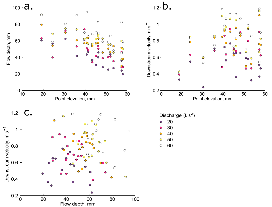
Figure 7. Relationships between downstream velocity, bed elevation, and water depth across all five discharges at each of the 18 measurement locations.
