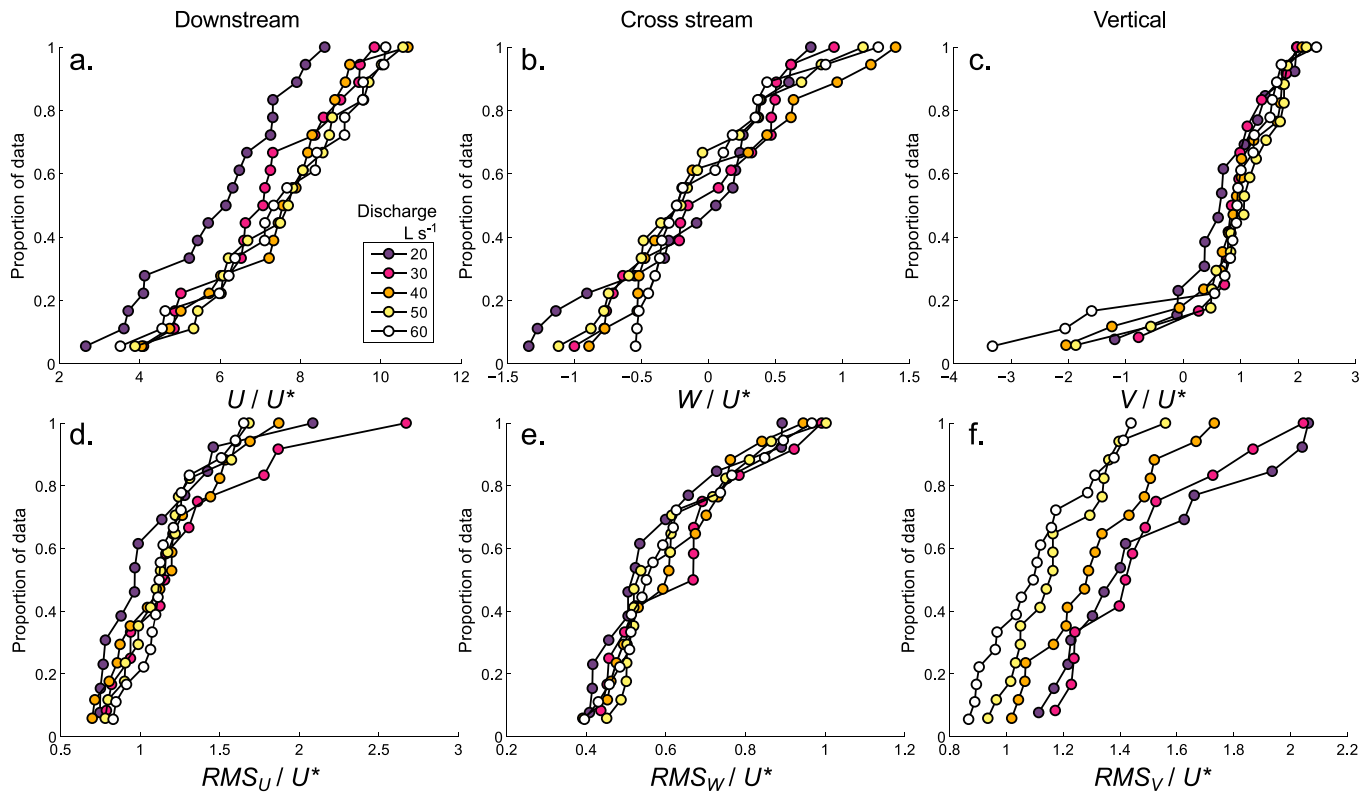
Figure 4. (a–c) Cumulative distributions of mean U (downstream), W (cross stream) and V (vertical) velocities for all 18 measurement locations at all 5 discharges. (d–f) Cumulative distributions of the RMS of velocity fluctuations. All data are normalized by U^* to enable comparison between different discharges.
