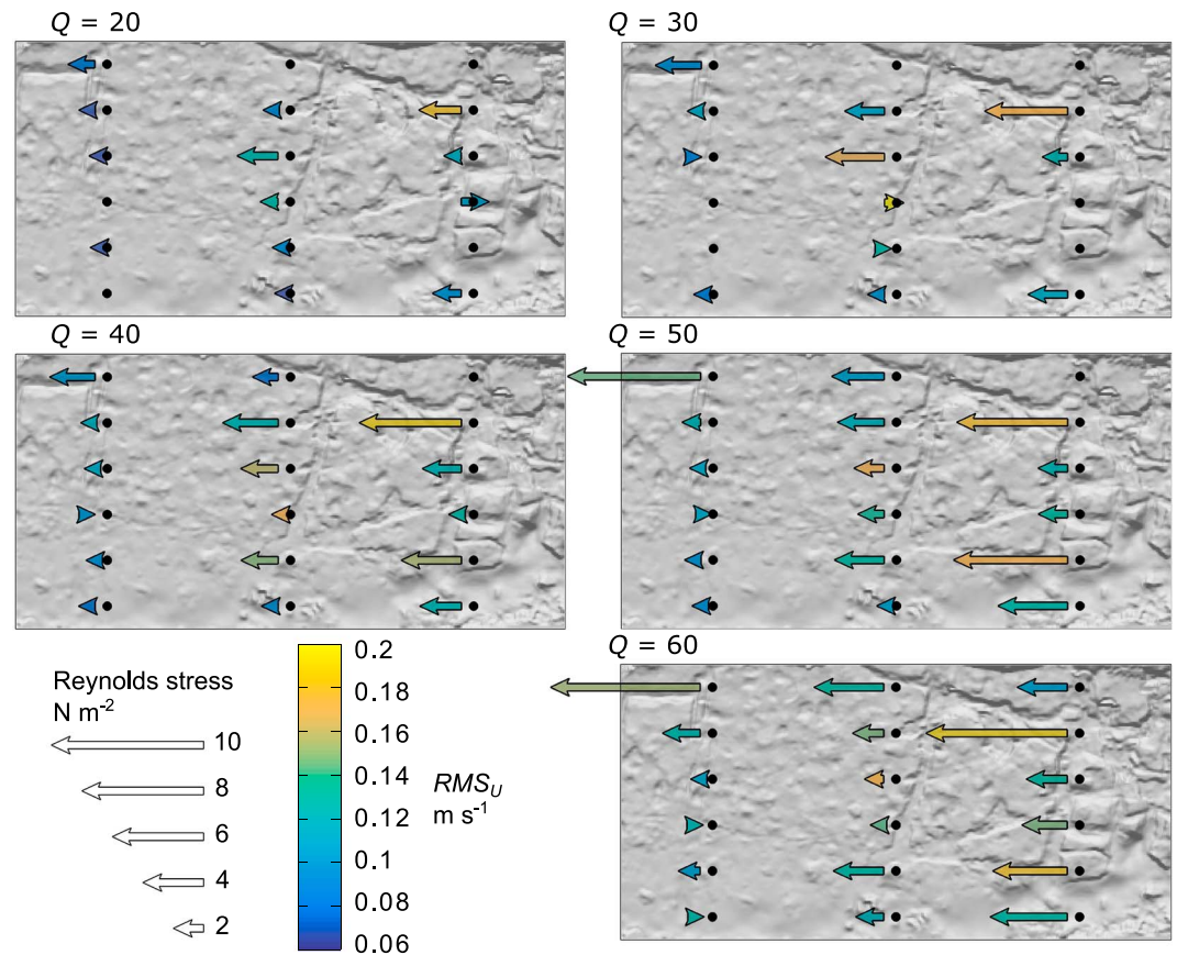
Figure 6. Maps of average Reynolds stress (arrow length) and RMS_U (colors) at each of the different discharges ( Q ). Upstream pointing arrows are negative Reynolds stresses. Absent arrows indicate that ADV data were not of sufficient quality to calculate Reynolds stress. Black dots show the measurement locations.
