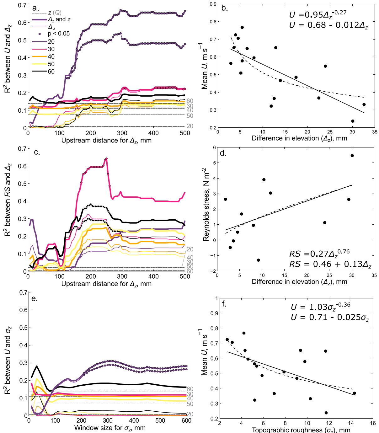
Figure 9. (a) R^2 values for relationships between the upstream difference in surface elevations ( \Delta_z ) and mean downstream velocity ( U ), using \Delta_z calculated over a range of upstream distances. (c) The same analysis but for Reynolds stress ( RS ) instead of U . (e) The same analysis as Figure 9a but characterizing topography using the standard deviation of elevations ( \sigma_z ) within a square window centered on the velocity measurement location. In all of Figures 9a, 9c, and 9e, thin lines are R^2 for the regression between the topographic index and the hydraulic data for each discharge; thick lines are R^2 for a regression that also incorporates the elevation of the measurement location (using the same color scheme for Q ), and dashed lines are for the regression between the point elevation and the hydraulic data. Circles indicate statistically significant relationships ( p < 0.05 ). (b, d, and f) The relationships between the topographic index and the hydraulic data for the highest R^2 in the previous panel. Dashed lines are power functions (top equation shown on each panel), and solid lines are linear relationships (bottom equation on each panel). In Figures 9b and 9f, Q = 20 L s^{-1} , and in Figures 9d Q = 30 L s^{-1} .
