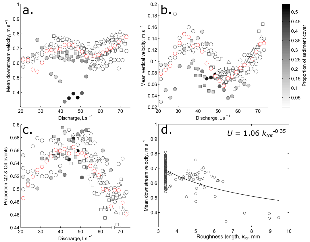
Figure 10. The impact of sediment cover on local velocities and flow structures; data are from all runs where sediment was introduced into the flume. The symbols show the discharge at which the run was initiated: circles, 20 \text{ L s}^{-1} ; squares, 35 \text{ L s}^{-1} ; and triangles, 50 \text{ L s}^{-1} . Figures show variation in (a) downstream velocity, (b) vertical velocity, and (c) proportion of time flow is in quadrants 2 and 4. Marker shade indicates the proportion of sediment cover in an area 40 \times 50 \text{ mm} upstream of the ADV location. Red markers are data from a control run with no sediment input. (d) The relationship between k_{\text{tot}} (equation (4)) calculated from a linear combination of bedrock and sediment roughness lengths, and downstream velocity. The fitted power law has R^2 = 0.33 , and the coefficient and exponent are significantly different to zero ( p = 0.05 ).
