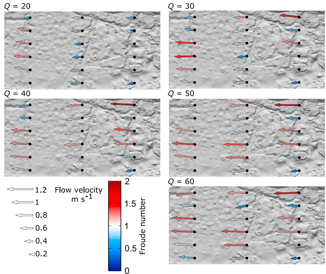
Figure 5. Vectors of downstream and cross-stream velocity under five different discharges ( Q ) between 20 and 60 \text{ L s}^{-1} . Arrow lengths show magnitude of resultant velocity, with all plots using the same scale. Arrow colors show local Froude number. Black dots show the measurement locations.
