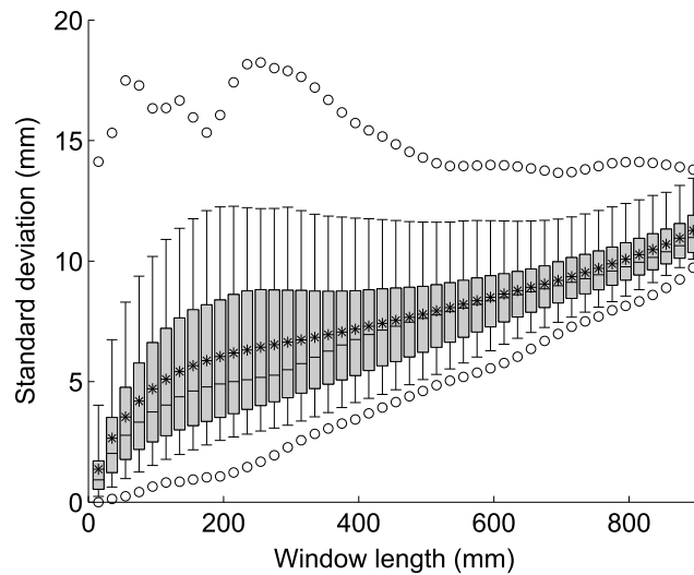
Figure 8. The standard deviation of the bedrock topography calculated using a square moving window of increasing length. Box plots show the minimum and maximum values (circles), 5th and 95th percentiles (whiskers), 25th, 50th, and 75th percentiles (box and dashed line), and mean (*). Lengths are for the flume tiles, multiply by 10 to get length scales for the field.
