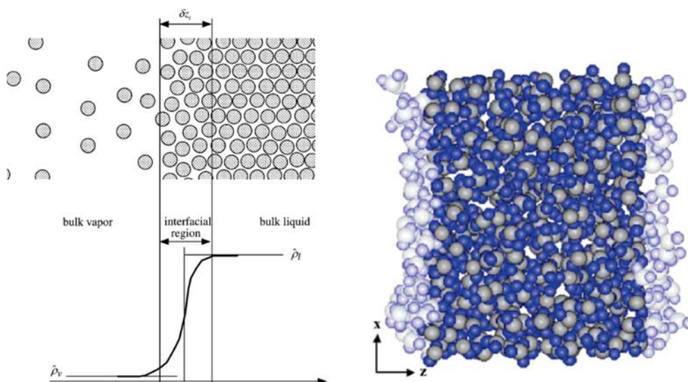
Figure 8: (left) Schematic of the gas-liquid water interface. (right) Molecular simulation of air-water interface showing two gas-water boundaries (perpendicular to the z-axis). The light colored water molecules indicate where the density is below 90% of the bulk liquid value. Reproduced with permission from [152] and [147] respectively.
