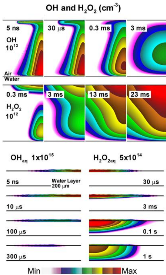
Figure 26: The time evolution of OH and H 2 O 2 densities in the (top) gas gap (initial gas mixture is 1 atm, N 2 /O 2 /H 2 O = 79.9/20/0.1 with water evaporation) and (bottom) 200 μm water layer. Densities of OH and OH (aq) are shown during the first pulse of -18 kV and interpulse afterglow. H 2 O 2 and H 2 O 2(aq) densities are shown accumulating after 3 successive pulses at 100 Hz (0, 100 ms, 200 ms) and during the terminal afterglow. The contours are plotted on a 3-decade log-scale with the maximum values noted in each frame. Reproduced with permission from [62].
