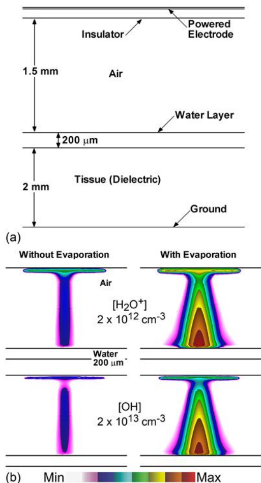
Figure 25: Dielectric barrier discharge filaments interacting with thin water layers over tissue (a) Geometry, showing 1.5 mm gas gap over a 200 \mu\text{m} water layer. The water evaporates into the gap. (b) Densities of \text{H}_2\text{O}^+ and \bullet\text{OH} in the discharge with and without evaporation of water vapor. The initial gas mixture is 1 atm, \text{N}_2/\text{O}_2/\text{H}_2\text{O} = 79.9/20/0.1 . Contours for \text{H}_2\text{O}^+ and \bullet\text{OH} are plotted on a log scale over three decades with the maximum density shown in each frame. Reproduced with permission from [62].
