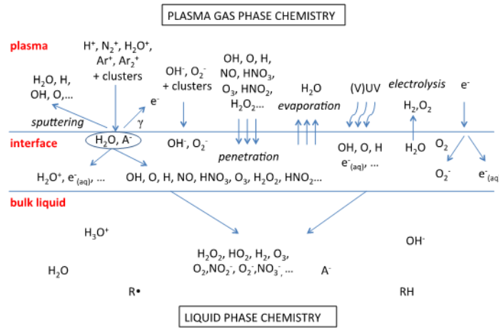
Figure 1: Schematic diagram of some of the most important species and mechanisms for an argon/humid air plasma in contact with water. Adapted from [24].
