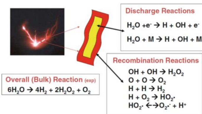
Figure 3: Schematic of the reaction chemistry in the model of Mededovic and Locke. Reproduced with permission from [38].
