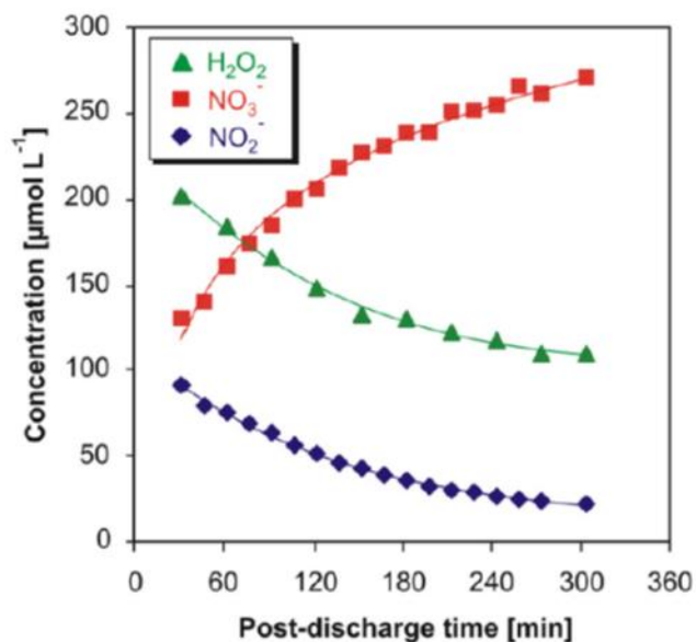
Figure 21: Post-discharge evolution of hydrogen peroxide, nitrite and nitrate in aqueous solution (pH 3.3) after treatment by an air plasma. Reproduced with permission from [486].
