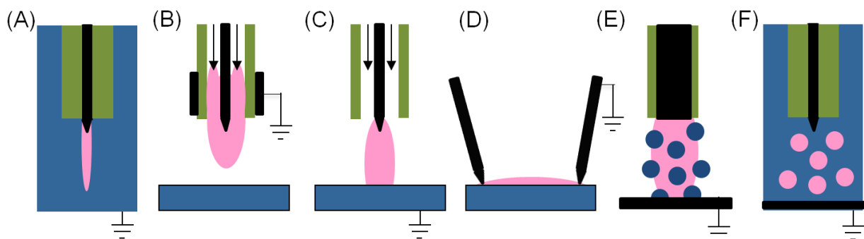
Figure 2: Schematic of different discharges used in plasma-liquid interactions: (a) Direct discharge in liquid, (b-d) gas phase discharges and (e-f) multiphase discharges. In more detail: (b) plasma jet without direct contact with liquid, (c) gas phase plasma with liquid electrode, (d) surface discharge, (e) gas phase plasma with dispersed liquid phase (aerosols) and (f) discharges in bubbles. Blue=liquid, pink=plasma, green=dielectric, black=metal electrodes.
