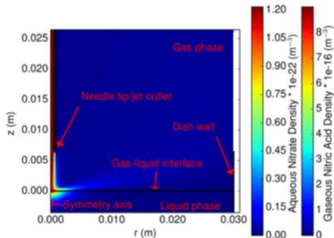
Figure 18: Model of the interaction of a reactive flow originating from the needle tip with relevant reactive species densities deduced from DBD plasmas. (top) The flow pattern in the gas and liquid phase. (middle) Distribution of the \text{HNO}_3 density in the gas and liquid phase. (bottom) Distribution of the \text{HNO}_3 density in the gas and liquid phase without liquid convection. Reproduced with permission from [323].
