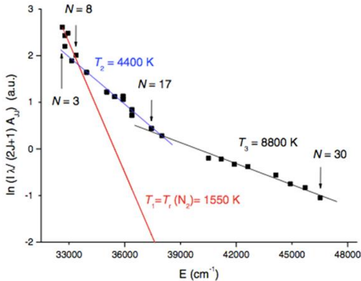
Figure 20: Boltzmann plot of the rotational distribution of OH(A) obtained from the emission spectrum of OH(A-X) from a discharge in a vapor bubble in water. Reproduced with permission from [453].
