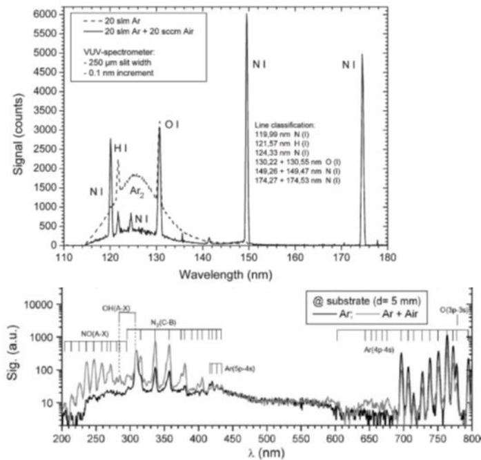
Figure 12: (top) VUV spectrum of an RF plasma jet without and with air admixture to the argon carrier gas. (bottom) UV-VIS spectra of an RF plasma jet without and with air admixture. Reproduced with permission from [257].
