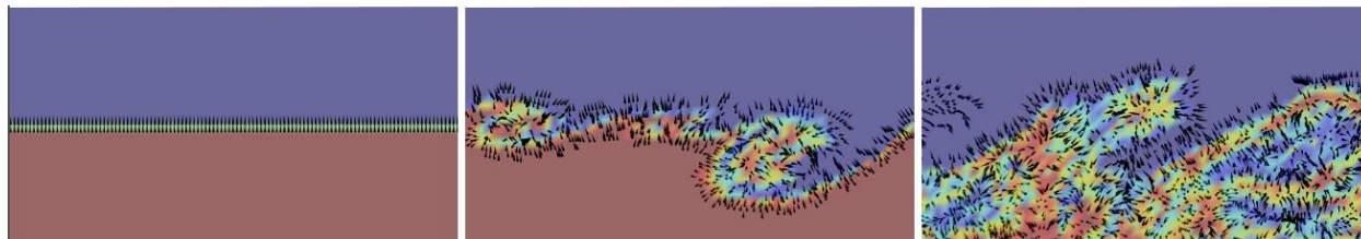
Figure 28: This sequence of images [599] shows the evolution of a multiphase temporal shear layer obtained from a model using a Lagrangian VOF approach [600]. Vectors point from the liquid into the gas and reflect the development of the Kelvin Helmholtz. While surface tension may stabilize the short wavelength instability, longer waveforms appear, stretch and distort the surface, creating new interface. Over the time interval shown vortices form and a transition to a fully turbulent interface occurs.
