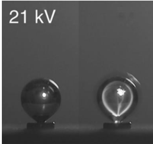
Figure 5: Filamentary surface discharge generated in a stable N_2 containing bubble at an orifice. The outer diameter of the orifice is 1.6 mm. Reproduced with permission from [69].
