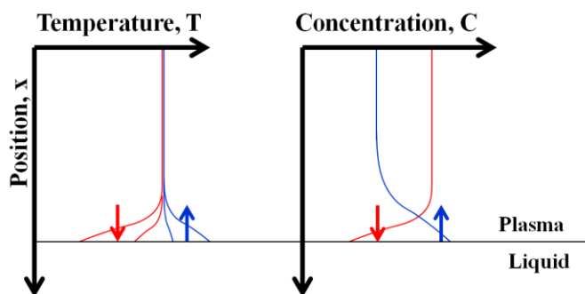
Figure 17: Schematics of temperature and concentration profiles above liquid in contact with plasma. The arrows indicate that both chemical species and energy can be transported in either direction depending on the local gradients.
