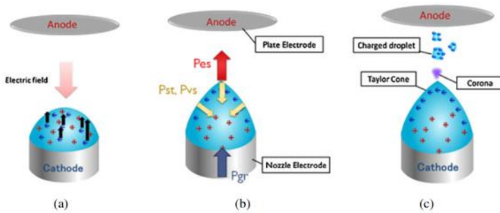
Figure 13: The formation of a Taylor cone: (a) initial state; (b) formation of cone; (c) corona discharge at the tip of the cone. Reproduced with permission from [296].
