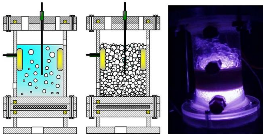
Figure 6: Schematic of a discharge with (left) bubbles and (right) foam with an image of the discharge in operation during foaming. Reproduced with permission from [118, 119].
