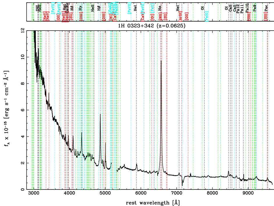
Figure A2. Keck LRIS optical spectrum shown as observed flux versus rest-frame wavelength. Emission lines labelled as in Fig. A1.
