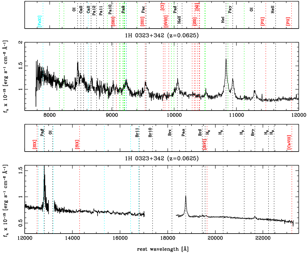
Figure A1. Gemini GNIRS near-IR spectrum shown as observed flux versus rest-frame wavelength. Emission lines listed in table 4 of Landt et al. (2008) are marked by dotted lines and labelled; black: permitted transitions, green: permitted Fe II multiplets (not labelled), red: forbidden transitions and cyan: forbidden transitions of iron (those of [Fe II] not labelled).
