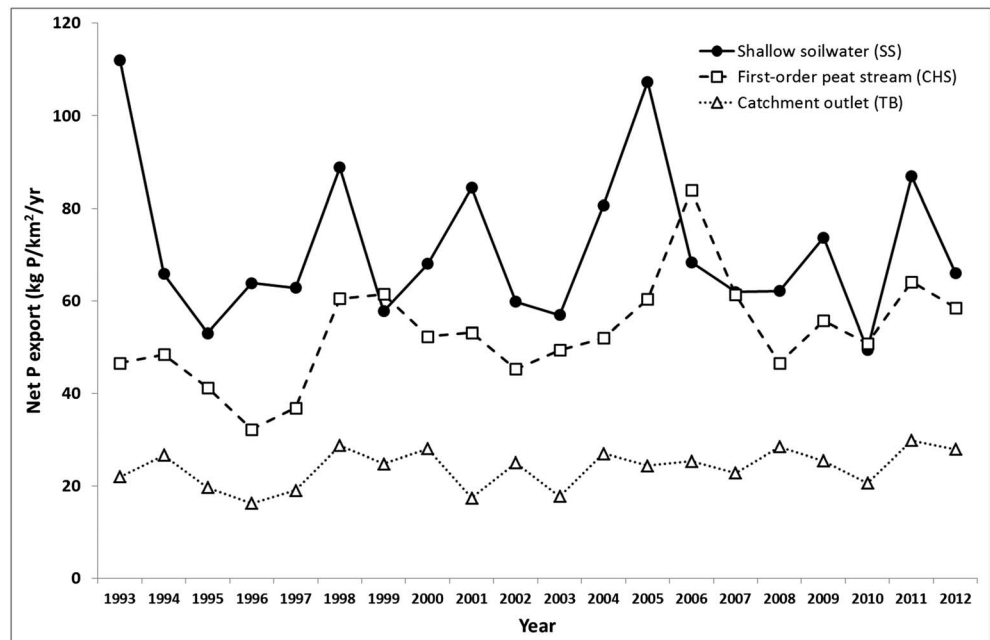
Figure 5. The time series of the fluvial export of total P over the course of the study. For discussion of errors on estimates see text.
