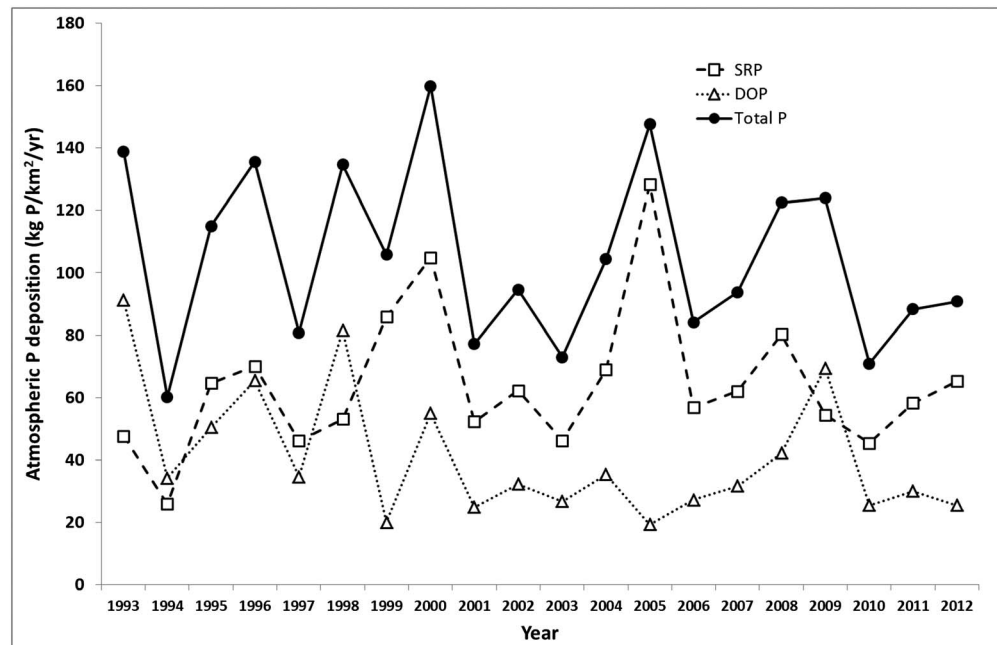
Figure 4. The time series of the atmospheric deposition of total P species at the soil source over the course of the study. For discussion of errors on estimates see text.
