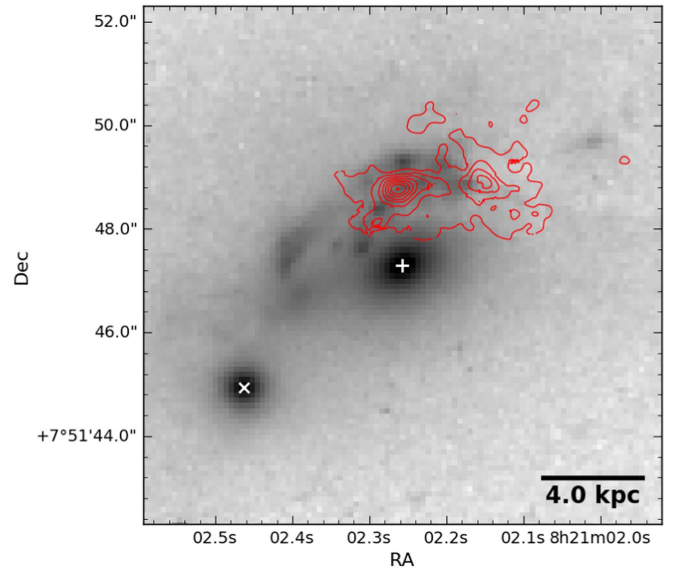
Figure 4. HST WFPC2 F606W imaging of the RXJ0821+0752 BCG overlaid with contours of the CO(3-2) emission obtained from ALMA. The + indicates the BCG nucleus, and the x indicates the centroid of a nearby galaxy that may be interacting with the BCG.
