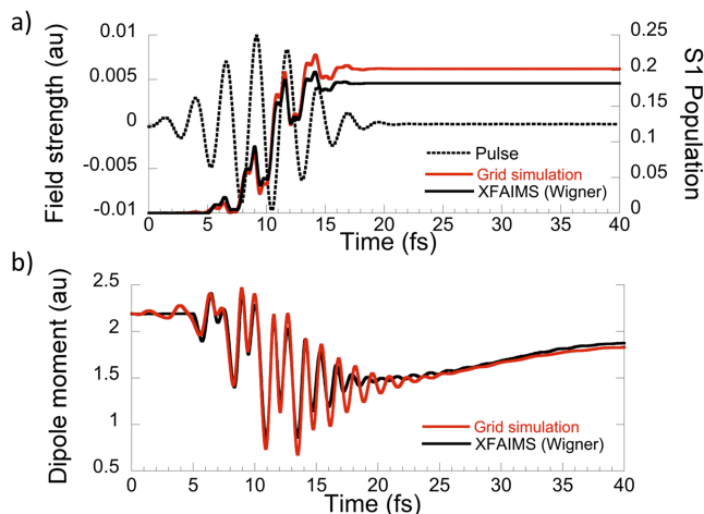
FIG. 3. (a) S_1 population induced by a 8.5 fs IR pulse polarized along the molecular axis ( f_0 = 0.01 a.u., FWHM = 8.46 fs, \omega = 0.0576 a.u., CEP = \pi ) computed on a grid and with XFAIMS. (b) Dipole moment along the molecular axis for the pulse of panel (a).
