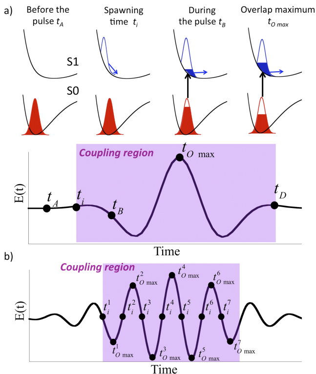
FIG. 1. Schematic representation of the spawning method during the pulse. The S_0 and S_1 potential energy surfaces of LiH are computed at the SA2-CASSCF(4/6)/6-31G level. In panel (a), only one TBF is spawned, at the time t_{O \max} , when the pulse is maximum. In panel (b), a new TBF is spawned every time the electric field reaches a maximum, twice per optical period. The area in purple represents the region where new basis functions can be spawned if required.
