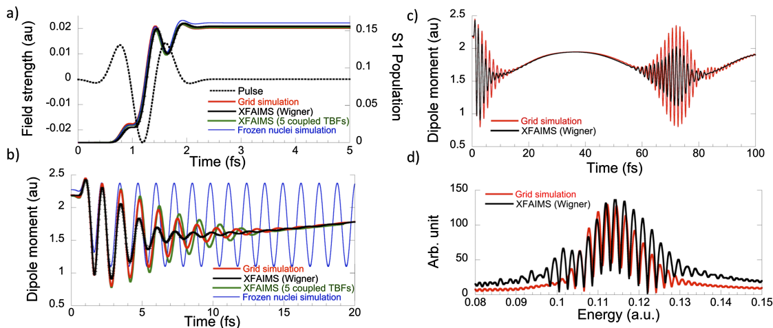
FIG. 2. (a) S_1 population induced by a resonant UV pulse polarized along the molecular axis ( f_0 = 0.025 a.u., FWHM = 0.84 fs, \omega = 0.127 a.u., CEP = \pi ) computed at frozen nuclei geometry, on a grid, and with XFAIMS, the latter for a set of 100 uncoupled initial conditions sampled from a Wigner distribution and for a set of 5 coupled TBFs. Standard error is given for the Wigner-sampled XFAIMS calculations. (b) and (c) Dipole moment along the molecular axis for the pulse of panel (a) in a time-window of 20 and 100 fs. (d) Fourier transform of the dipole moment in panel (c).
