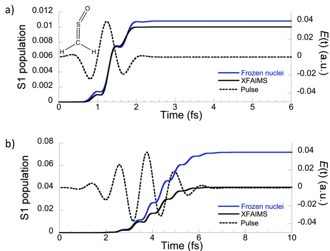
FIG. 4. (a) S_1 population induced by a 0.85 fs resonant UV pulse polarized perpendicularly to the molecular axis ( f_0 = 0.04 a.u., FWHM = 0.85 fs, \omega = 0.12 a.u.). The sulfine molecule is shown in the inset. (b) Same as (a) for a 2.54 fs pulse ( f_0 = 0.04 a.u., FWHM = 2.54 fs, \omega = 0.12 a.u.).
