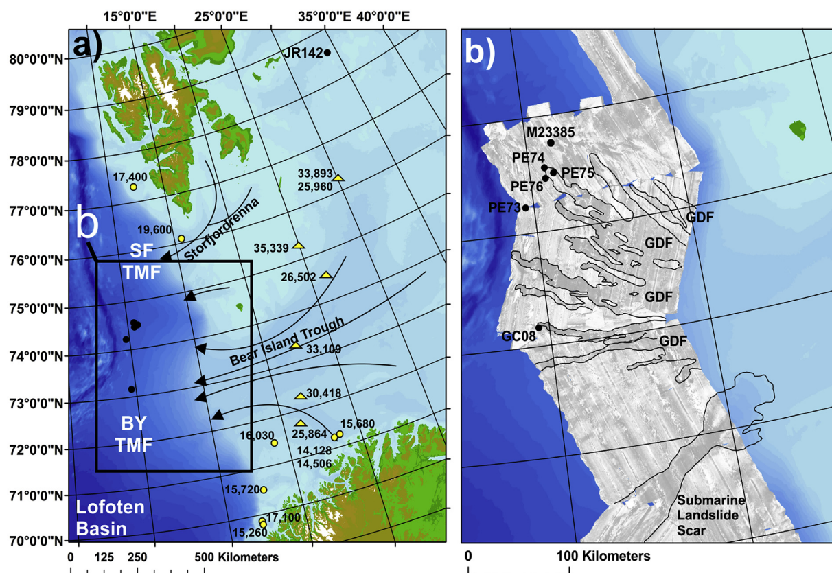
Fig. 1. Regional setting of the Bear Island Trough-Mouth Fan. a) Core locations (black dots) shown with respect to Last Glacial Maximum ice flow direction inferred from the orientation of streamlined seafloor bedforms (Winsborrow et al., 2010). SF TMF = Storfjorden Trough-Mouth Fan. BY TMF = Bear Island Trough-Mouth Fan. Yellow triangles show dates from till units giving maximum age estimates for the onset of the last glacial advance and dots triangles show dates from glaciomarine sediments giving minimum estimates for the onset of deglaciation (Winsborrow et al., 2010). b) Bear Island Trough-Mouth Fan with GLORIA long range side-scan sonar imagery – superimposed. Core positions are labelled. Glacigenic debris-flows (GDF) and the Bjørnøya submarine landslide are identified using the GLORIA imagery. (For interpretation of the references to colour in this figure legend, the reader is referred to the web version of this article).
