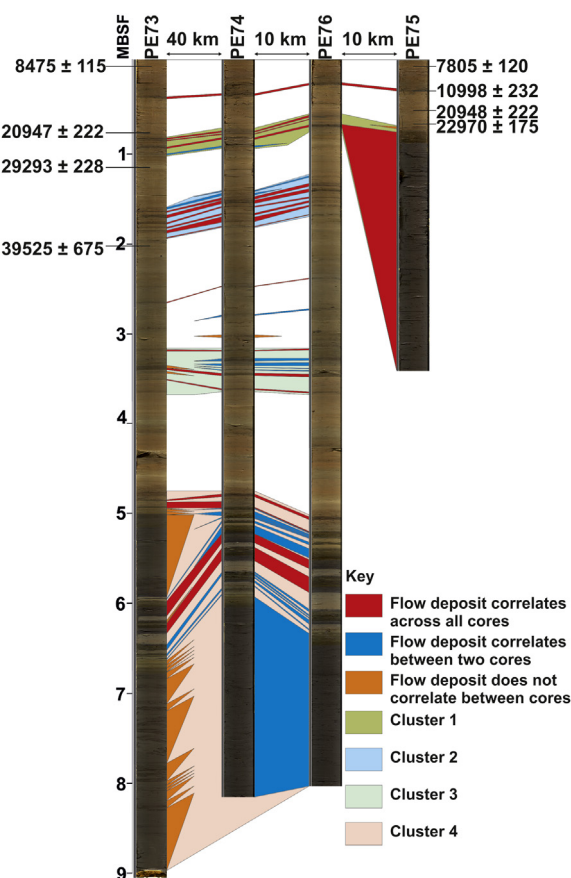
Fig. 7. Core correlations between cores PE73, PE74, PE75 and PE76. Distances between the cores and radiocarbon dates from cores PE73 and PE75 are shown. MBSF = Meters Below Sea Floor. Four clusters of distal debris-flow muds correlate well across the three long cores. Few deposits from glacial debris-flows occur outside of these main clusters.
