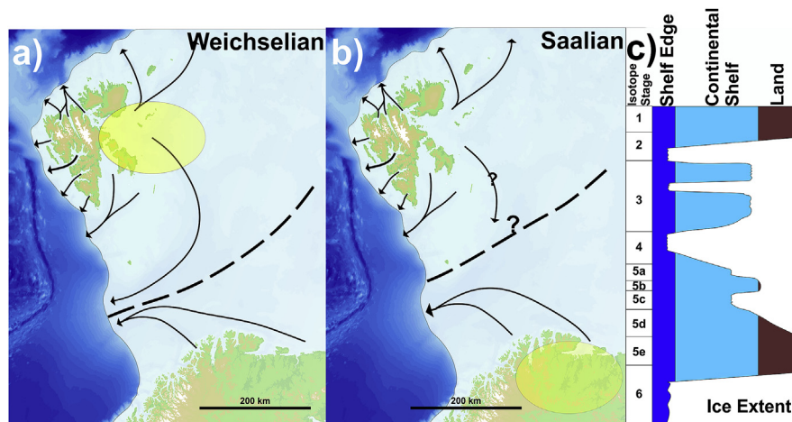
Fig. 10. Ice sheet chronology for the Bear Island Trough during the last 140 ka. a) Palaeo ice-flow directions during the Weichselian with respect to the Bear Island Trough-Mouth Fan. During the Weichselian the northern end of the fan is dominated by an ice dome (in yellow) east of Svalbard. b) Palaeo ice-flow directions during the Saalian glaciation. During the Saalian the northern end of the fan is dominated by an ice dome (in yellow) associated with northern Scandinavia. c) A schematic plot of glacial advance and retreat in the Bear Island Trough. Ice advances are in white, areas currently below sea level are in blue and areas currently above sea level are in brown. (For interpretation of the references to colour in this figure legend, the reader is referred to the web version of this article).
