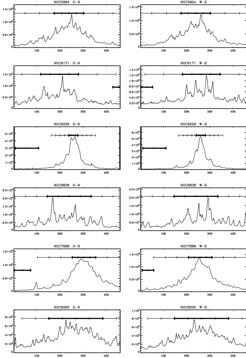
Fig. 2.— Observed light profiles of the 24 GCGs. The profiles were obtained by adding flux along the dispersion axis. The x-axis is in pixels and the y-axis is in flux units. In each panel, the upper bars indicate various extraction windows with the thick upper bar equal to the size of the core radius. Lower thick bars represent extraction windows of the background sky selected well away from the globular cluster.
