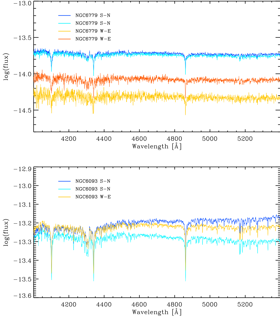
Fig. 4.— Differences in spectral shape between individual spectra for the same GC. The spectra of NGC 6779 (upper panel) show a difference in continuum flux level between exposures, while the spectra of NGC 6093 show a difference in the spectral slope.
