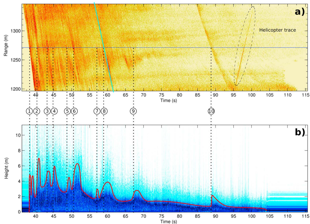
Figure 4. (a) GEODAR data from avalanche #0017 taken at the distance of FMCW B (blue horizontal line at 1271 m range). The turquoise-marked surge from Figure 3 is shown for reference. (b) FMCW flow height data acquired at cavern B. An approximate flow height h is drawn in red. Vertical dotted lines help to match flow height variations with GEODAR line features. For detailed description see text. FMCW data are shifted by -1 s relative to GEODAR time due to the transverse displacement of the FMCW system.
