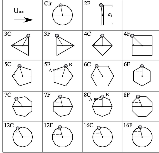
FIGURE 12. Schematic diagrams indicating the location of the separation point above the centreline, marked by a circle, and the separation angle \theta_s , marked by \angle , as determined at \text{Re} = 1.0 \times 10^4 .
