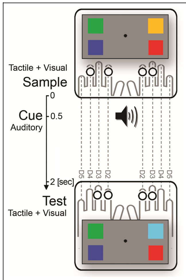
Figure 1. Stimulation procedure and task. A bimodal (tactile–visual) sample set was presented before an auditory retrocue, which was followed by a bimodal test set. Participants memorized the locations of the tactile sample stimuli (symbolized by black dots) and the colors of the visual sample stimuli on one task-relevant side (left or right, varied across blocks). On each trial, the pitch of the retrocue indicated whether the memorized tactile or visual stimuli (unpredictably 50%) had to be retained and compared with the test stimulus set.
