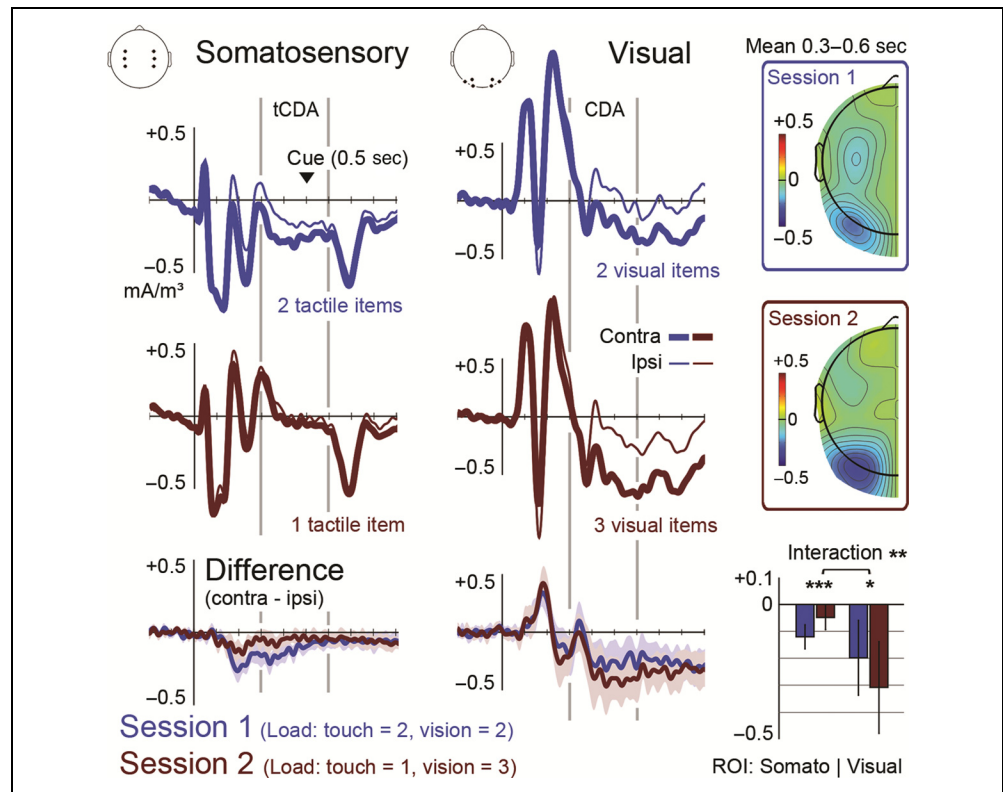
Figure 3. Grand mean CSDs in the early period of the retention delay measured at somatosensory (tCDA, left) and visual ROIs (CDA, right) in Session 1 (blue) and Session 2 (brown). CSDs were recorded contralateral (thick line) and ipsilateral (thin line) to the memorized sample set. The bottom panels show contra- minus ipsilateral difference waves, with shaded areas indicating 95% within-subject CIs for tests against zero (i.e., no lateralized effect). CSDs were collapsed across the factor levels of Cued modality. Note that negativity is plotted downwards and that different scales were used for somatosensory and visual CSDs (as indicated by the length of the y axes representing \pm 0.5 \text{ mA/m}^3 ). Bar graphs display mean amplitudes of the tCDA/CDA averaged for the time period before neural responses were triggered by the retrocue (300–600 msec after sample onset); error bars represent 95% CIs for tests against zero. Topographical maps illustrate the scalp distribution of the central tCDA and the posterior CDA components that were elicited during the concurrent maintenance of tactile and visual sample stimuli in Session 1 and Session 2.
