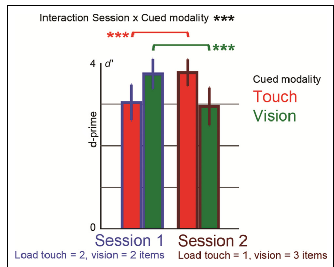
Figure 2. Behavioral performance, quantified in d' , in the tactile task (red bars) and visual task (green bars), and in Session 1 (blue outlines) and Session 2 (brown outlines). *** p < .001 .
