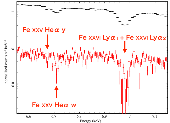
Figure 9. HEG spectra of GX 13+1 from 1st order (black) and 3rd order (red).
