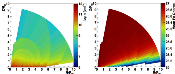
Figure 6. Distribution of density (left) and Fe ionisation state (right) for the diverging wind geometry. The accelerating flow gives higher density material close to the disc compared to the constant velocity outflow model in Fig. 1, giving lower mean ionisation state.
