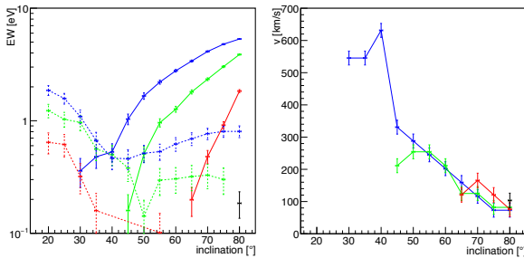
Figure 8. As in Fig. 3, but for the diverging wind model. The lower ionisation state means that there is also a contribution from the inter-combination line of Fe xxv Heα γ (black) at the highest inclinations.
