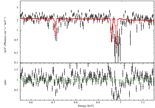
Figure 11. The model (red) and HEG 3rd order spectrum (black). The best fit inclination angle is i = 80^\circ . This gives roughly the correct column of Fe XXV and XXVI at low velocity, but fails to match the observed higher velocity blue wing to the absorption features.
