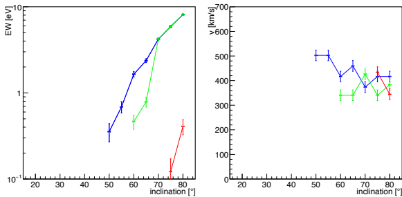
Figure 3. Left panel: EW of the absorption lines as a function of inclination angle, Fe xxv (He \alpha w , red) and Fe xxvi (Ly \alpha_2 , green and Ly \alpha_1 , blue). The EW of all absorption lines increases strongly at higher inclination, showing the assumed equatorial disc wind geometry. The Doppler wings (with width set by turbulent velocity) of the two H-like absorption lines start to merge for inclinations above 70° so above this we show the total EW of the two lines. Right panel: the blue shifted absorption line velocity for each ion species. This clearly shows the assumed constant velocity structure of the radial streamline.
