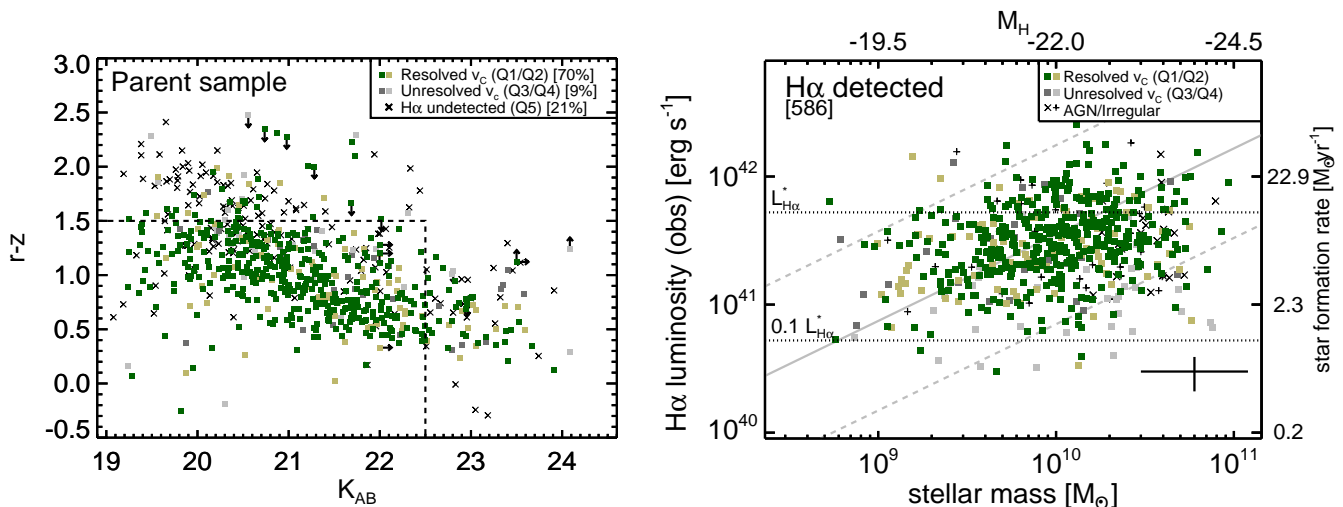
Figure 1. Left: The r-z colour versus observed K_{AB} magnitude for the parent KROSS sample. The square symbols represent the 586 H\alpha detected sources used for dynamical analyses in this work; with green symbols representing sources which have spatially-resolved velocity measurements (dark/light corresponds to quality 1/quality 2 [Q1/Q2]; see Section 3.4) and grey symbols representing sources that have spatially-unresolved velocity measurements (dark/light corresponds to quality 3/quality 4 [Q3/Q4]). The dashed lines show the selection criteria for the highest priority targets. Right: Observed H\alpha luminosity versus stellar mass (scaled from M_H ; top axis; Section 2.2) for the H\alpha detected targets. The symbols are coloured as in the left panel. Systematic error bars are shown in the bottom right. The solid line shows the “main sequence” of star forming galaxies at z=0.85 (Speagle et al. 2014; see Section 2.3) and the grey dashed lines are a factor of five above and below this. The dotted lines show 0.1 \times and 1 \times L_{H\alpha}^* for this redshift (Sobral et al. 2015). The targets have a median star-formation rate of 7 M_{\odot} \text{yr}^{-1} and are representative of typical star-forming galaxies.
