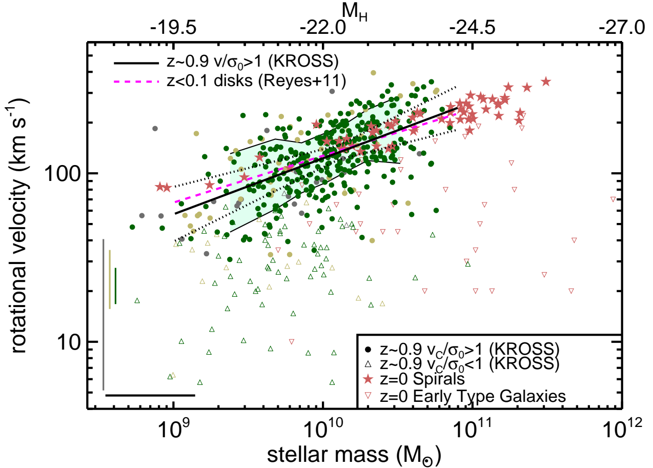
Figure 6. Rotational velocity ( v_C ) as a function of estimated stellar mass (scaled from M_H ; top axis) for KROSS galaxies that are rotationally dominated (circles) and dispersion dominated (triangles). The symbol colours are as described in Figure 1. From left to right, the three vertical lines show the median uncertainty (in log space) for quality 3, 2 and 1 sources, respectively, and the horizontal line shows the systematic uncertainty for converting M_H to stellar mass. The shaded region shows the running \approx 0.2 dex (68 per cent) scatter on the velocities of the rotationally-dominated sources and the bootstrap 1\sigma uncertainty (dotted lines; see Section 4.2). This is in excellent agreement with equivalent H \alpha observations of local disks (Reyes et al. 2011) and stellar observations of local spiral galaxies from Romanowsky & Fall 2012. Dispersion-dominated galaxies do not follow this trend, similar to the z=0 early-type galaxies from Romanowsky & Fall 2012.
