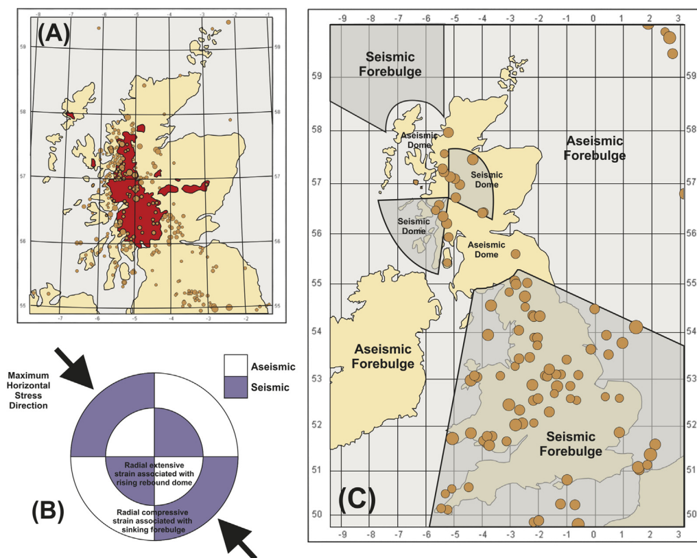
Fig. 4. (a) Scottish seismicity (earthquake epicentres orange circles) and the extent of the Younger Dryas ice cap (red) (after Musson, 2007). (b) Radial strain quadrant scheme of Muir-Wood (2000) for deglaciation seismogenesis theory (after Musson, 2007). (c) Seismic and aseismic quadrants for deglaciation seismogenesis (Muir-Wood, 2000) applied to historic UK earthquakes with M_L > 4.0 (orange circles) (after Musson, 2007). (For interpretation of the references to colour in this figure legend, the reader is referred to the web version of this article.)
