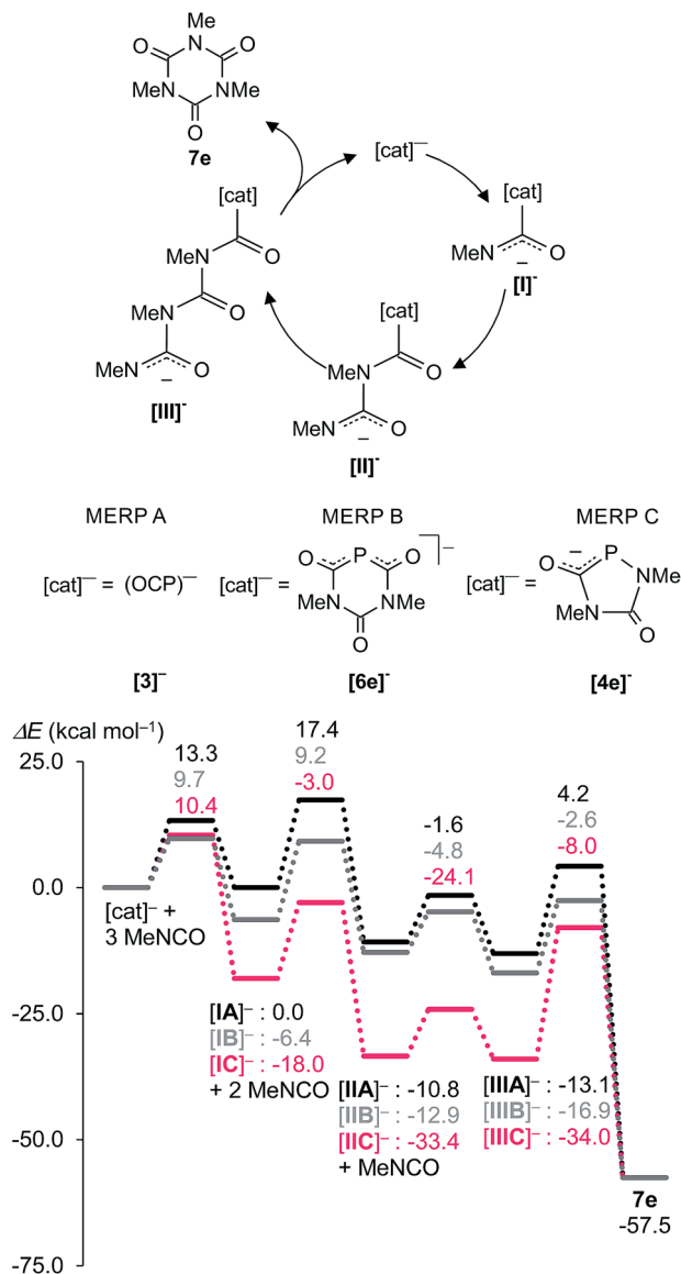
Fig. 8 Proposed catalytic cycle leading to 7e on the MERPs A, B, and C computed at the B3LYP/aug-cc-pVDZ//B3LYP/6-31+G* level. MERP A (black) corresponds to the reaction catalysed by the (OCP) - anion [3] - , MERP B (grey) to the reaction catalysed by the six-membered heterocyclic anion [6e] - , and MERP C (magenta) stands for the trimerization reaction catalysed by the five-membered heterocyclic anion [4e] - . The notation of the intermediates: [I] - , [II] - and [III] - indicate adducts between [cat] - and one, two and three isocyanate molecules. Na + was included as a counter cation in the computations but is not shown.
