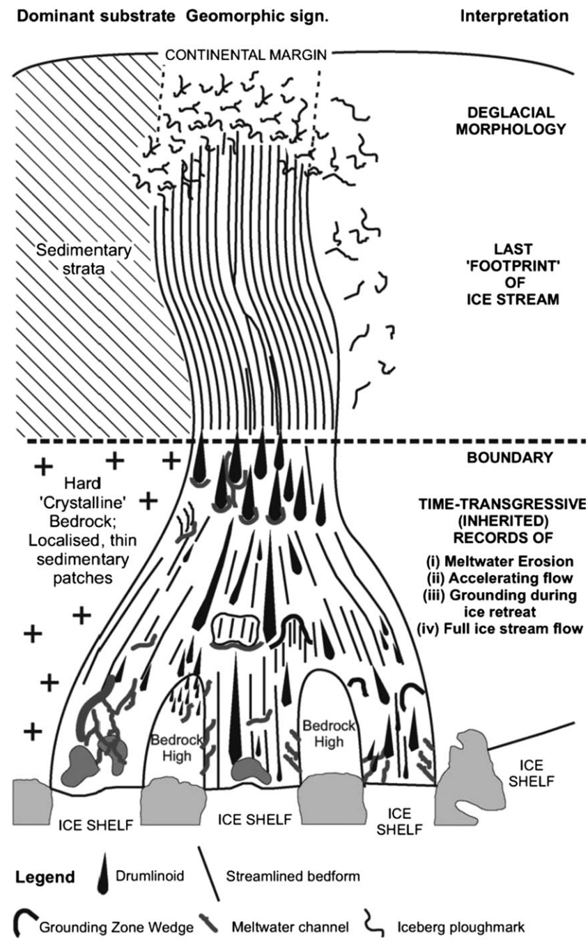
Figure 10. Conceptual model of palaeo-ice stream geomorphology on the west Antarctic continental shelf (from Graham et al. , 2009) highlighting the complex time-transgressive landform assemblage, particularly in ice stream onset zones. Reproduced by permission of Elsevier.
