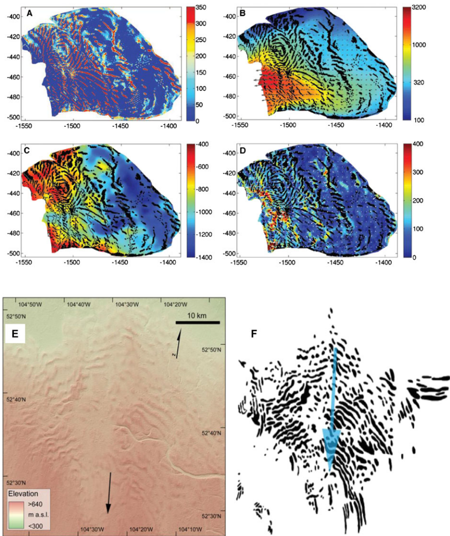
Figure 16. (a) Inverted basal shear stress for Thwaites Glacier, West Antarctica (in kPa). (b) Observed ice surface speed with black patches ('traction ribs') showing locations where basal shear stress (in a) is >100 kPa. (c) Bed elevation and traction ribs (in black). (d) Gradient of the hydraulic potential (in pascals per meter), with traction ribs (in black). (e) Example of a cluster of low-amplitude rib-like ridges aligned transverse to ice flow on a digital elevation model of the Buffalo Ice Stream corridor in Saskatchewan (see Ross et al. , 2009 and Stokes et al. , 2016b). (f) Black patches show the location of the central area of rib-like features in (e). (a-d) taken from Sergienko and Hindmarsh (2013; reproduced by permission from The American Association for the Advancement of Science) and (e-f) taken from Stokes et al. (2016). [Colour figure can be viewed at wileyonlinelibrary.com ]
