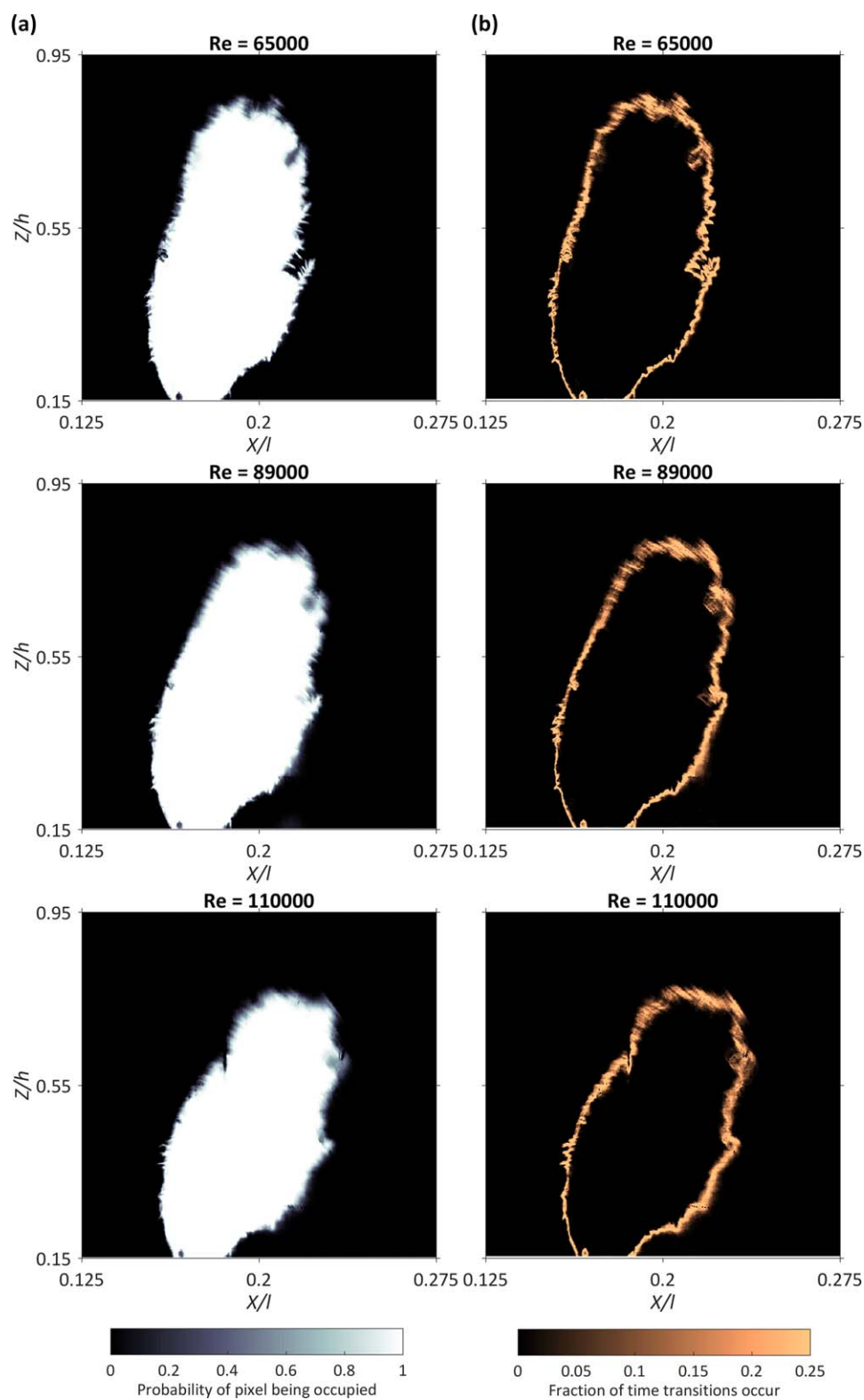
Figure 4. Time-averaged plant position for Re = 65,000 (row 1), Re = 89,000 (row 2), and Re = 110,000 (row 3), showing (a) the probability of individual pixels being occupied through time (column 1), and (b) the fraction of time transitions occur (column 2), highlighting zones of greatest motion on the upper and leeward sides.
