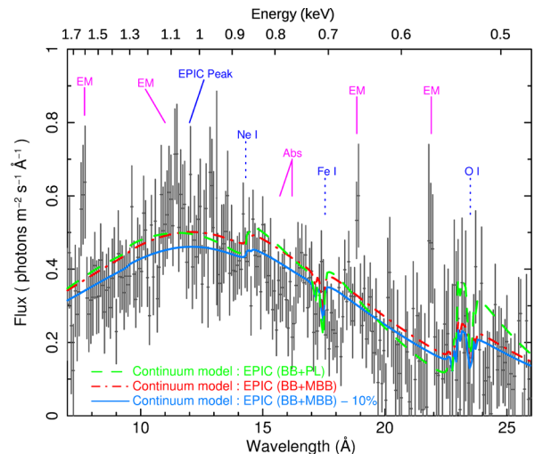
Figure 4. RGS stacked spectrum with the overplotted EPIC best-fitting continuum model (see Table 2). The solid blue line shows the RGS-fitted continuum with free normalization as only free parameter. The wavelengths of expected absorption lines produced by the Galactic absorber (Pinto et al. 2013) and the \sim 1 keV peak seen in the EPIC spectrum are shown by blue dashed lines. Some clear emission- (EM) and absorption- (Abs) spectral features are marked with solid magenta lines.
