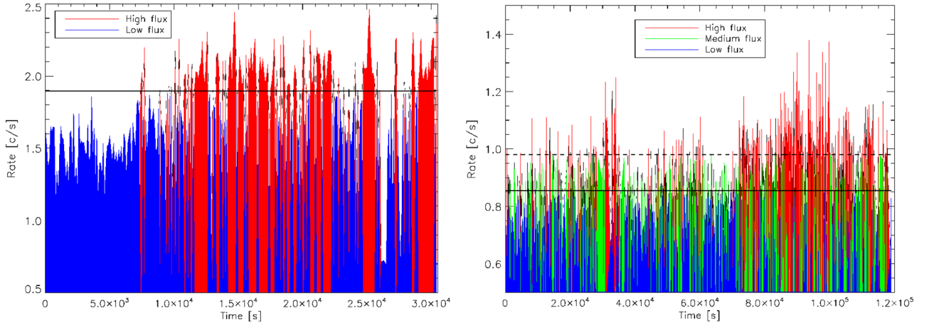
Figure A2. EPIC/pn 0.3–10 keV light curves of the first (left) and second (right) observations both with time bins of 100 s. Flux thresholds were chosen in order to have comparable statistics. For more detail see the text.
