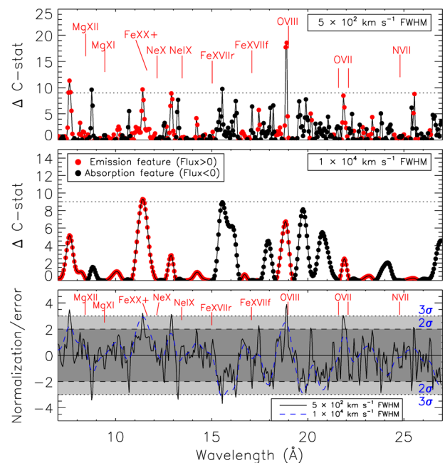
Figure 5. \Delta C-statistics obtained by fitting a Gaussian spanning the 7–27 Å wavelength range with increments of 0.05 Å. \Delta C = 2.71, 4.00 and 9.00 refer to 1.64 \sigma (90 per cent), 2 \sigma (95.45 per cent) and 3 \sigma (99.73 per cent) confidence levels. We tested the effects of using two different line widths: 500 km s -1 ( \sim RGS resolution, top panel) and 10 000 km s -1 (medium panel). Red and black points refer to emission and absorption lines, respectively. The ratio between the normalization of the Gaussian and its error is shown in the bottom panel. The rest-frame wavelengths of some relevant transitions are labelled. More detail on the line significance is reported in the text.
