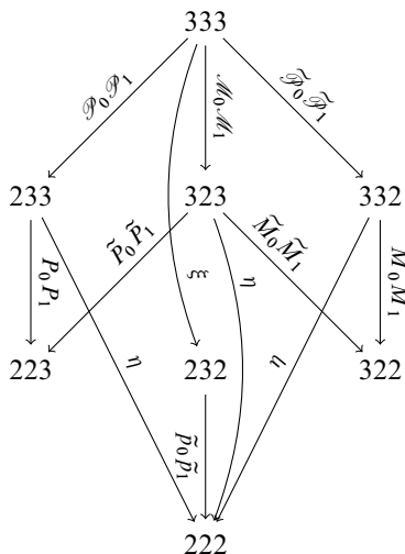
Figure 7: The framed flow category \mathcal{C}_3
