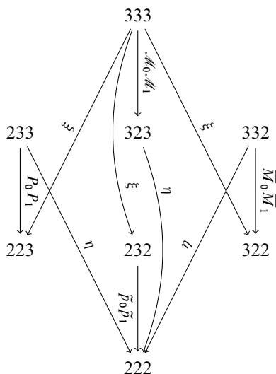
Figure 8: The framed flow category \mathcal{C}_4 . Note that the associated cochain complex is in Smith normal form; see Section 6.
