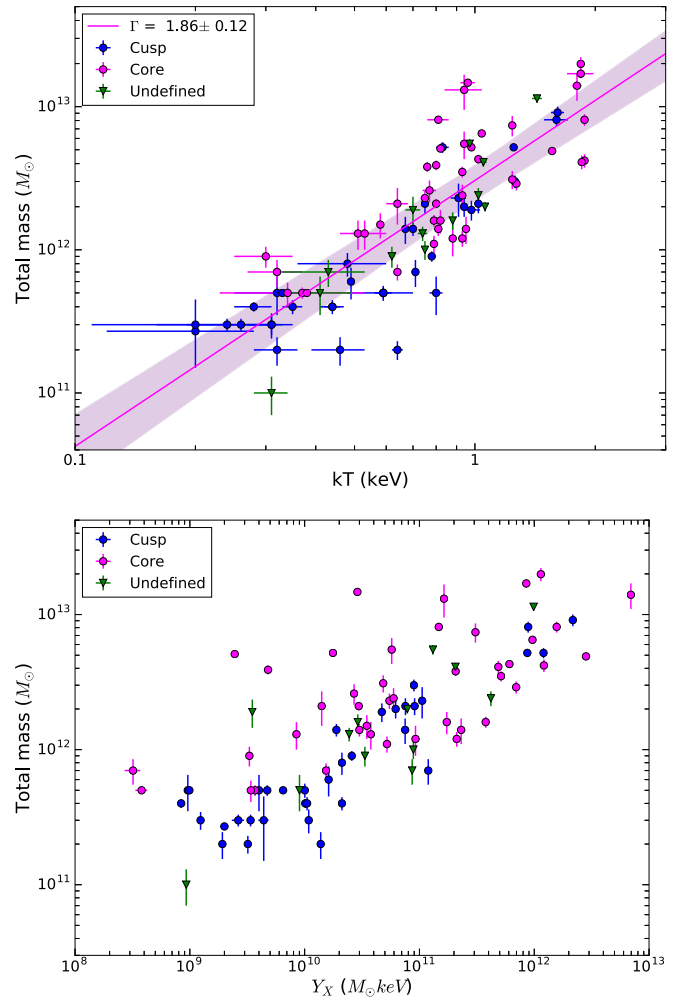
Figure 6. X-ray scaling relations for galaxies with an X-ray core/cusp. The fits in magenta were obtained from X-ray core galaxies only.
