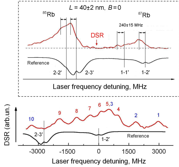
Fig. 4. Experimental DSR spectrum for L = 40 \pm 2 nm recorded at B = 2.15 kG (upper trace) and B = 0 reference spectrum (lower trace). The inset: DSR and reference spectra at B = 0 showing -240 \pm 15 MHz red shift with respect to ^{87}\text{Rb} F_g = 1 \rightarrow F_e = 1, 2 and ^{85}\text{Rb} F_g = 2 \rightarrow F_e = 2, 3 reference frequencies.
