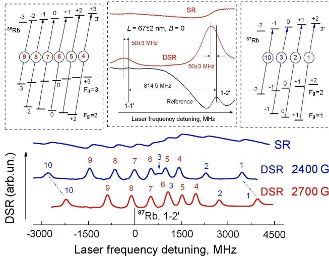
Fig. 2. Selective reflection spectrum (SR, upper line) and its derivative (DSR) for L = 67 \pm 2 nm, recorded at B = 2.4 kG (middle curve), and 2.7 kG (lower curve). For labeling, see the upper left- and right-side insets presenting \sigma^+ -polarized transition diagrams for ^{85}\text{Rb} and ^{87}\text{Rb} , respectively. The upper middle inset: B = 0 spectra (from top to bottom: SR, DSR, and reference) exhibiting \sim 50 MHz red shift with respect to F_g = 1 \rightarrow F_e = 1, 2 transitions of ^{87}\text{Rb} .
