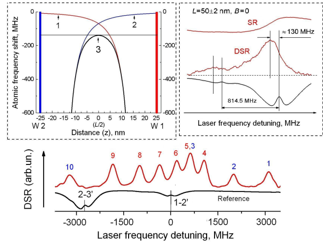
Fig. 3. Experimental DSR spectrum for L = 50 \pm 2 nm recorded at B = 2.15 kG. Upper-right inset: B = 0 spectra (from top to bottom: SR, DSR, and reference), exhibiting \sim 130 MHz red shift with respect to ^{87}\text{Rb} F_g = 1 \rightarrow F_e = 1, 2 reference frequencies. Upper-left inset: the estimate of distance-dependent vdW red shift; the horizontal line tangent to an overall curve 3 marks the minimum shift value ( -130 MHz).
