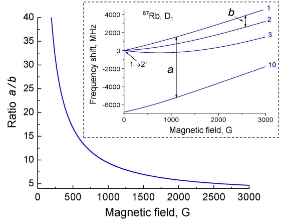
Fig. 5. B -field dependences of DSR frequencies exploited for realization of two ways to determine the magnetic field value (see text).
