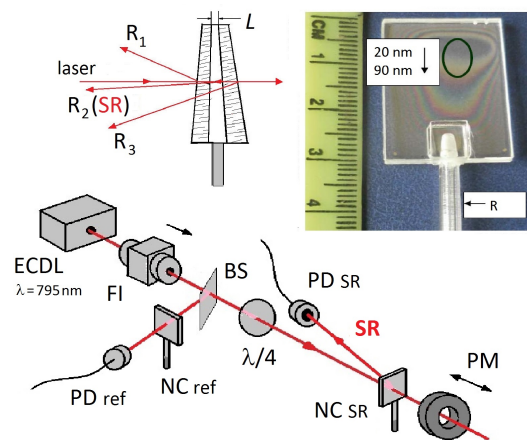
Fig. 1. Layout of the experimental setup: (ECDL) cw laser, (FI) Faraday isolator, (BS) beam splitter, (NC) Rb nanometric-thickness cell inside an oven, (PM) permanent magnet, (PD) photodetector, ( \lambda/4 ) quarter-wave plate ("SR" and "ref" denote selective reflection and reference channels). Upper right inset: photograph of the NC, oval marks 20 – 90 nm region. Upper left inset: geometry of the 3 reflected beams. The beam (SR) propagates in the direction of R_2 .
