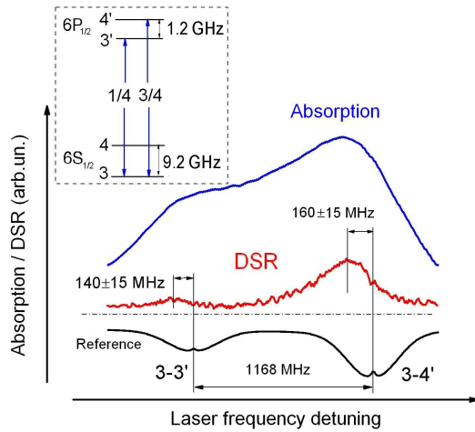
Fig. 7. Absorption spectrum (upper trace) and DSR spectrum (middle trace) recorded on Cs D_1 line and for L \approx 52 \pm 3 nm, P_L \approx 0.2 mW, NC temperature \approx 170 °C. The lower trace is the reference spectrum obtained with an auxiliary NC with L = \lambda , with VSOP resonances serving as ^{133}\text{Cs} F_g=3 \rightarrow F_e=3,4 transition frequency markers [14]. Inset shows the diagram of these transitions with indication of their relative intensities.
