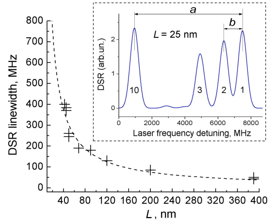
Fig. 6. Dependence of DSR linewidth \gamma_{DSR} versus L . The inset: four DSR peaks of the ^{87}\text{Rb} D_1 line at L = 25 nm and B = 2 kG; \gamma_{DSR} \approx 600 MHz. The inset shows theoretical spectrum calculated using dependences of the frequency shifts and transition probabilities versus magnetic field, see [12].
