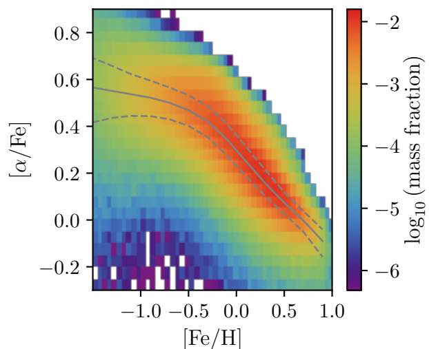
Figure 1. Two-dimensional histogram of the mass-weighted [\alpha/\text{Fe}]-[\text{Fe}/\text{H}] distribution of all ‘disc stars’ associated with the 133 galaxies identified as broad analogues of the Milky Way in terms of their stellar mass and morphology (see Section 2.2.1) at z=0 in Ref-L100N1504. The overplotted solid line shows the median [\alpha/\text{Fe}] in bins of \Delta[\text{Fe}/\text{H}]=0.2 , dashed lines show the interquartile range.
