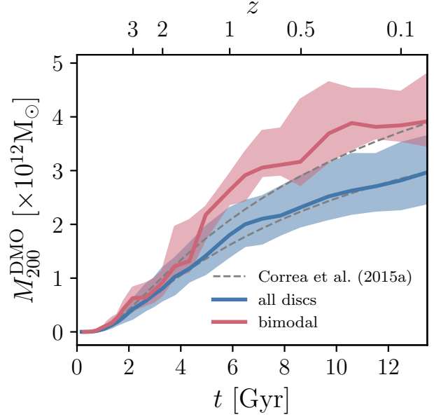
Figure 9. The mass accretion history, M_{200}(t) , of haloes identified in the DMONLY-L100N1504 simulation. The thick curves corresponds to the median, whilst the shaded regions denote the interquartile range. The blue curve corresponds to the partner haloes of all 133 galaxies in our Milky Way-like sample, whilst the red curve corresponds to the partner haloes of the 6 galaxies exhibiting bimodality in [\alpha/\text{Fe}] at fixed [\text{Fe}/\text{H}] . Dashed curves meeting the two median curves at z = 0 show the typical accretion history, as parametrised by (Correa et al. 2015a), of haloes with these z = 0 masses. Haloes which host galaxies exhibiting [\alpha/\text{Fe}] bimodality have systematically different dark matter accretion histories
