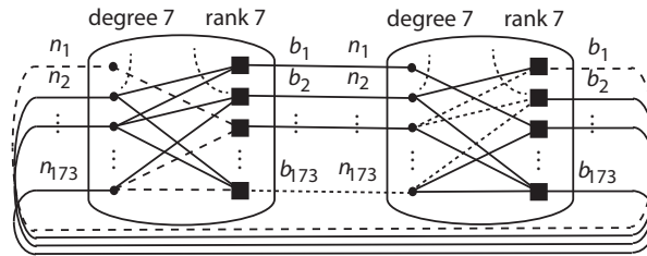
Figure 9: Our regular, uniform bipartite graph construction.
