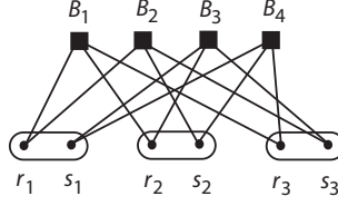
Figure 8: The unique [3, 2] -transversal design.
