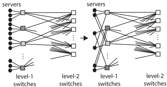
Figure 6: Building a switch-centric DCN via Method B .
