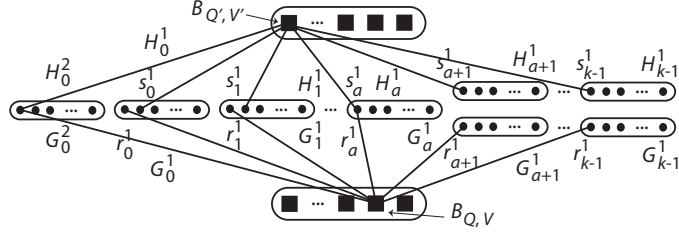
Figure 7: The basic set-up in Case (a)(i).
