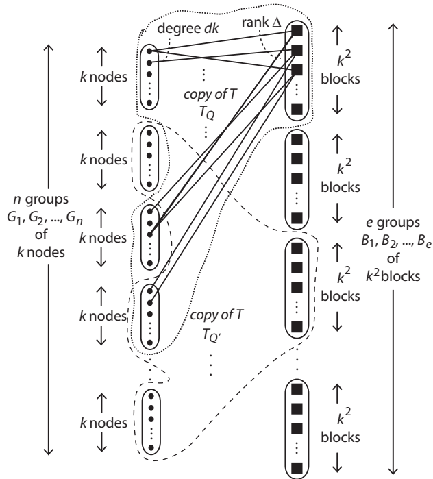
Figure 3: Amalgamating H_0 and T to get H .
