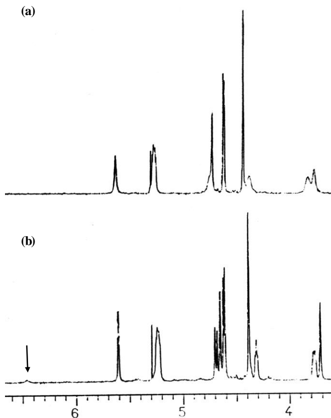
Fig. 1: partial ^1\text{H} NMR spectrum of the binuclear compound
