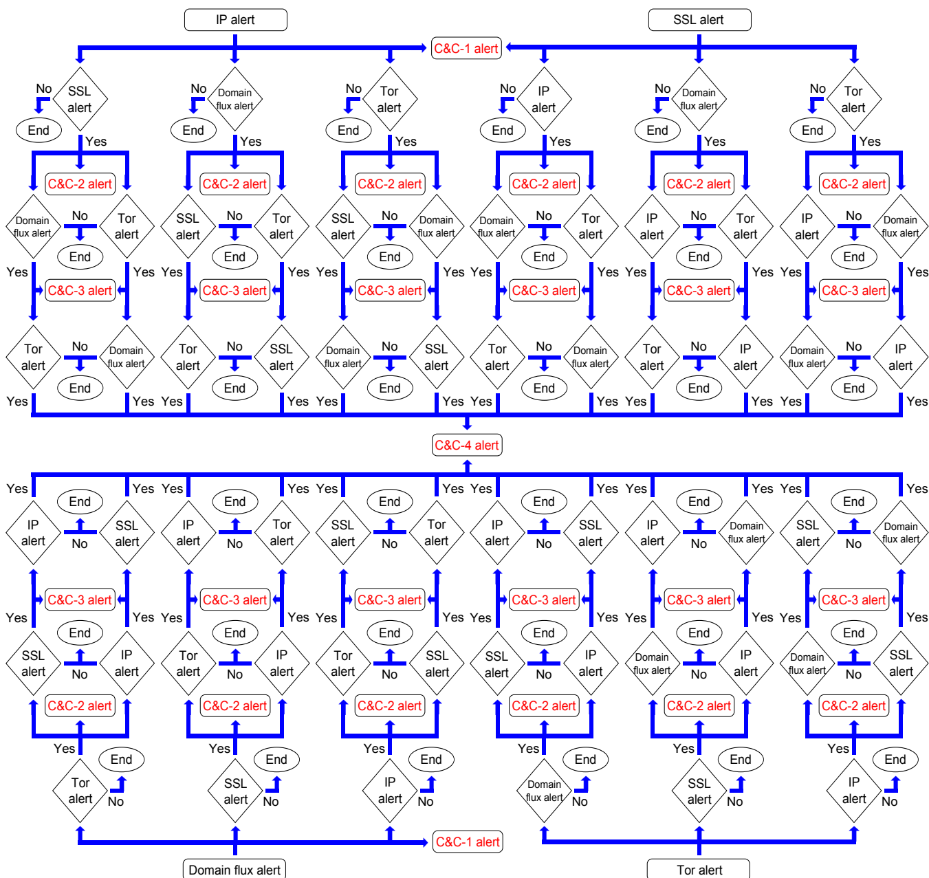
FIGURE 8. The architecture of the correlation framework.
