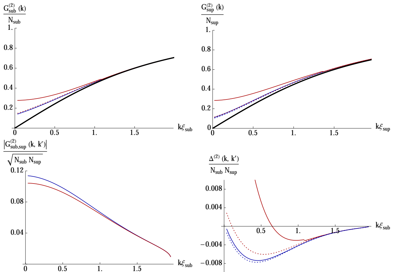
Figure 4. Density-density correlation function for a waterfall in BEC, with Mach number in the supersonic region M_{\text{sup}} = 4 (close to that reported in [21]). The plots in the upper row show the autocorrelation G^{(2)}(k) in the subsonic (left panel) and supersonic (right panel) regions, while the lower left panel plots the cross-correlation G^{(2)}(k, k') . The lower right panel shows instead the difference appearing in inequality (23). The variously colored curves correspond to different initial temperatures (in the frame of the condensate) of the incident v -modes: T_{\text{in}} = 0 (blue curves) and T_{\text{in}} = 2T_H (red curves – the kinks appearing in these are numerical artifacts due to assuming that the scattering is trivial above \omega_{\text{max}} , the maximum frequency at which (u, u) phonon pairs are produced). In the upper plots, the thick black curves show the autocorrelation in vacuum, which must be subtracted before insertion into inequality (23). The solid curves are those that are actually observed; by contrast the dotted curves are those that would result if the measurements were able to distinguish u - and v -modes, and only the occupation numbers of u -modes were to appear in all expressions. When the initial temperature T_{\text{in}} = 2T_H , the pollution of the density measurements by the presence of v -modes dramatically affects the observations of G^{(2)}(k) in the subsonic and supersonic regions (and, therefore, also the computed value of \Delta^{(2)} ), as can be seen by comparing the solid and dotted red curves in the upper plots and in the lower right plot. Indeed, since the u - v coupling is small, the occupation numbers of u -modes remain essentially the same whether or not there is an initial thermal state, as indicated by the fact that the dotted red curves are almost the same as the blue curves in the upper plots.
