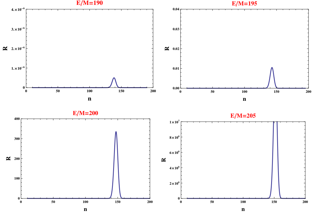
Figure 2. Multi-particle decay rates eq. (5.2) of a highly-energetic single-particle state into n scalars plotted as function of n . The four sub-figures show the energy E fixed at 190M_h , 195M_h , 200M_h and 205M_h and we used \lambda = 1/8 . There is a sharp exponential dependence of the peak rate on the energy. The peak multiplicities n \sim 150 in these examples are not far from the maximally allowed values at the edge of the phase space n_{\max} \sim E/M_h .
