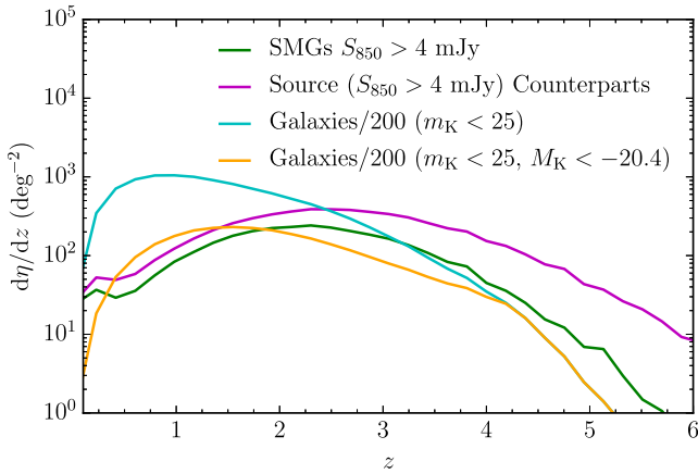
Figure 2. Predicted average redshift distributions from our 50 \times 4 \text{ deg}^2 fields for S_{850\mu\text{m}} > 4 \text{ mJy} galaxies (green line), the counterparts (see the text) of sources with S_{850\mu\text{m}} > 4 \text{ mJy} extracted from the simulated submm imaging (magenta line), flux-limited sample of K -band-selected galaxies (cyan line) and a volume-limited sample (for z < 4 ) of K -band-selected galaxies (orange line). The latter two lines have both been divided by a factor of 200 for presentation purposes. All magnitudes are in the AB system.
