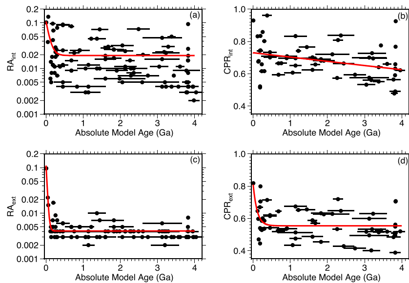
Figure 11. Interior (top) and exterior (bottom) rock abundance (left) and CPR (right) as a function of age for 113 selected craters. Error bars show the uncertainties in the absolute model ages.
