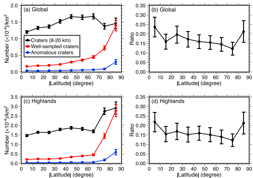
Figure 5. (a) Areal density of LU78287GT craters with: 8 \leq \text{diameter/km} \leq 20 (black), the subset with Miniature Radio Frequency (Mini-RF) coverage \geq 0.9 (red), and the subset with Mini-RF coverage \geq 0.9 and \Delta\text{CPR} \geq 0.1 (blue). (b) Fraction of well-sampled craters that are CPR-anomalous as a function of latitude, folding together both hemispheres. (c) Areal density of LU78287GT craters over the highlands with: 8 \leq \text{diameter/km} \leq 20 (black), the subset with Mini-RF coverage \geq 0.9 (red), and the subset with Mini-RF coverage \geq 0.9 and \Delta\text{CPR} \geq 0.1 (blue). (d) Fraction of well-sampled craters over the highlands that are CPR-anomalous as a function of latitude, folding together both hemispheres. The error bars in (a) and (c) represent 1\sigma statistical uncertainties assuming a Poisson distribution, and the error bars in (b) and (d) follow from the straightforward propagation of errors.
