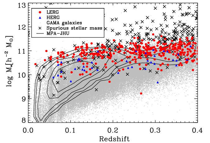
Figure 2. The stellar mass as a function of redshift for a subset ( z < 0.4 ) of the full GAMA II sample (grey points) and radio galaxies coloured according to their final classification: LERG (red) and HERG (blue). Contours of SDSS galaxies with stellar mass estimates from MPA-JHU are shown for comparison. The crosses mark GAMA galaxies with spurious stellar masses (see Section 3.2), which we remove from our analysis.
