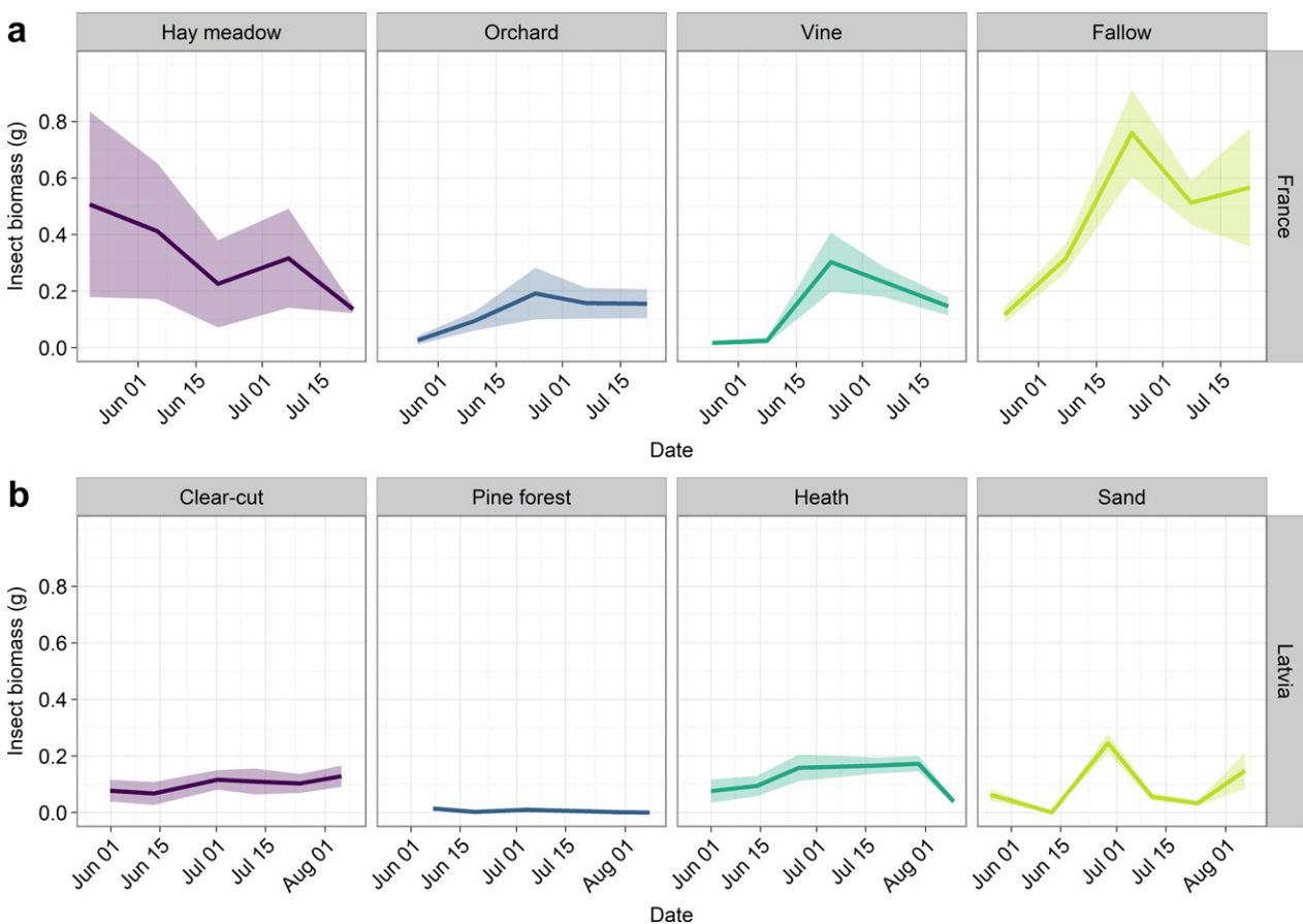
Figure 2. Insect biomass (g per transect) as a function of calendar date and land-use in (a) France and (b) Latvia. Lines show mean observed biomass per transect \pm se. [Colour figure can be viewed at wileyonlinelibrary.com ]
