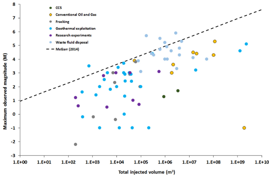
Fig. 97. M_{MAX} vs. total injected volume for the 69 cases of induced seismicity for which data are available. The upper-bound magnitude limit proposed by McGarr (2014) on the basis of theoretical considerations is also plotted.
