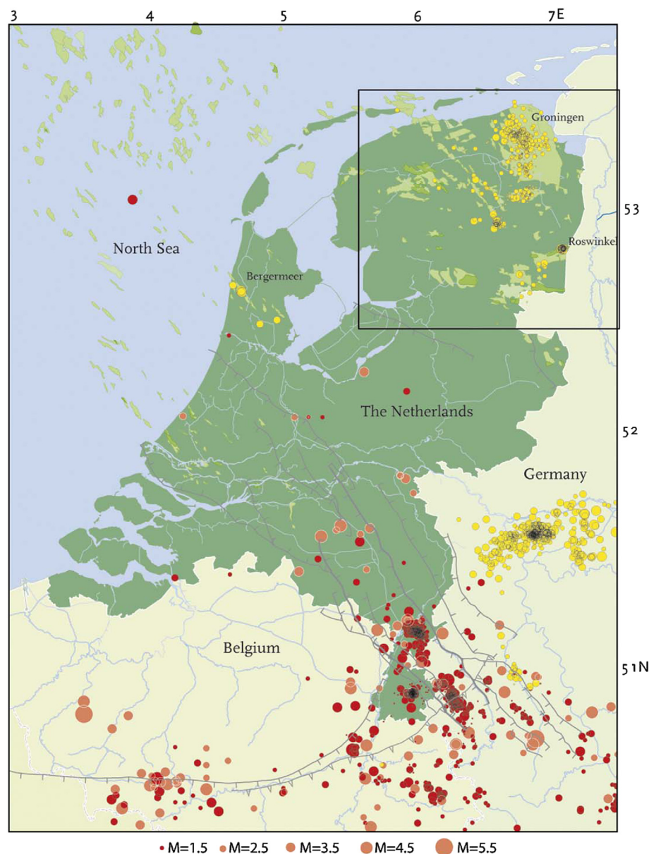
Fig. 33. Seismicity in the Netherlands and surrounding region since 1900. Red circles: natural tectonic earthquakes; yellow circles: suspected induced earthquakes (usually mining or gas exploitation); gray solid lines: mapped faults in the upper-North-Sea formation; light green: gas fields. Detail of boxed region shown in Fig. 34. (From van Eck et al. (2006).)
