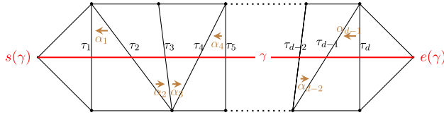
Fig. 1. Denoting the vertices in the quiver corresponding to an arc \tau_i of the triangulation also by \tau_i z , the string corresponding to the arc \gamma is given by w(\gamma) = \tau_1 \xleftarrow{\alpha_1} \tau_2 \xrightarrow{\alpha_2} \tau_3 \xleftarrow{\alpha_3} \tau_4 \xrightarrow{\alpha_4} \tau_5 \cdots \tau_{d-2} \xrightarrow{\alpha_{d-2}} \tau_{d-1} \xleftarrow{\alpha_{d-1}} \tau_d .
