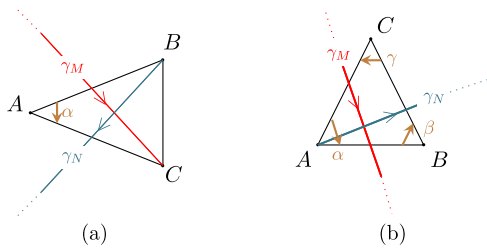
Fig. 5. Local configurations of crossings of \gamma_M and \gamma_N induced by the module M crossing the module N , corresponding in (a) to a crossing as in Definition 3.1 (2) and in (b) to Definition 3.1 (3).
