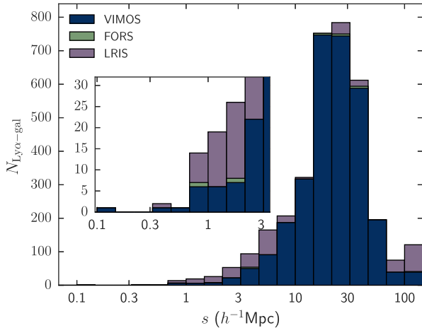
Figure 2. Number of LBG-sightline pairs ( N_{\text{Ly}\alpha\text{-L BG}} ) as a function of pair separation, s . The filled blue histogram shows the VIMOS detected galaxies, the green histogram the additional FORS detected galaxies, and purple the added LRIS galaxies (with the three histograms stacked to form the total). The inset shows a zoom in of the pair count histograms at small separation.
