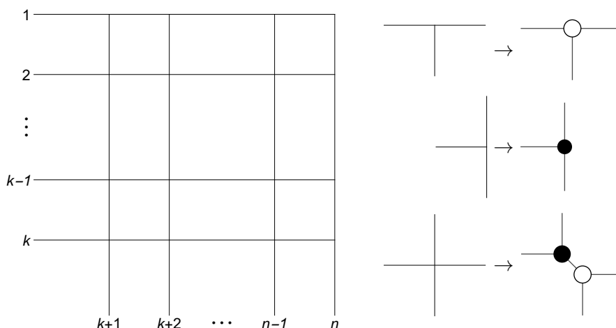
Figure 14. Postnikov diagram for n -point N^{k-2} MHV amplitude in \mathcal{N} = 4 SYM.
