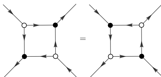
Figure 3. Square move equivalence relation SYM.
