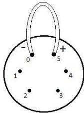
Figure 18. The worldsheet configuration describing a 1-loop 4-point amplitude in 4d ambitwistor string theory.
