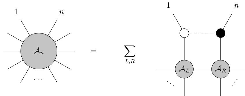
Figure 5. Tree-level BCFW recursion relations in \mathcal{N} = 8 SUGRA.
