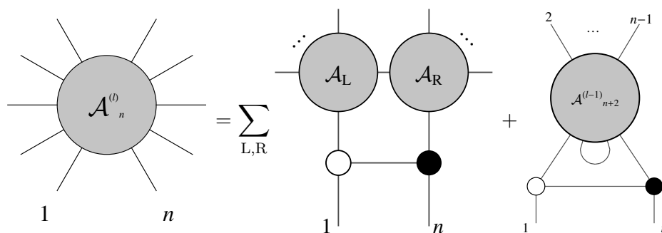
Figure 2. Loop-level BCFW recursion for planar \mathcal{N} = 4 SYM.
