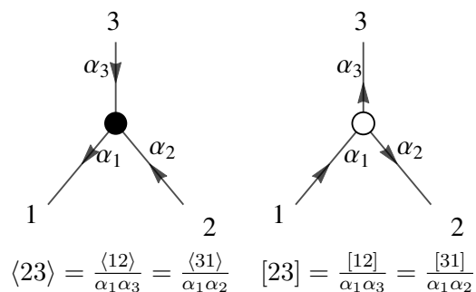
Figure 21. Relations between spinor bracket factors at each vertex of an on-shell diagram in \mathcal{N} = 8 SUGRA.
