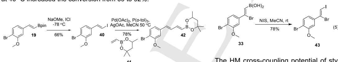
Scheme 6. Iterative cross coupling cycle to furnish aryl dienyl boronate ester 41 .
