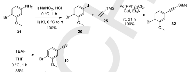
Scheme 4. Successful route towards alkyne 10 .
