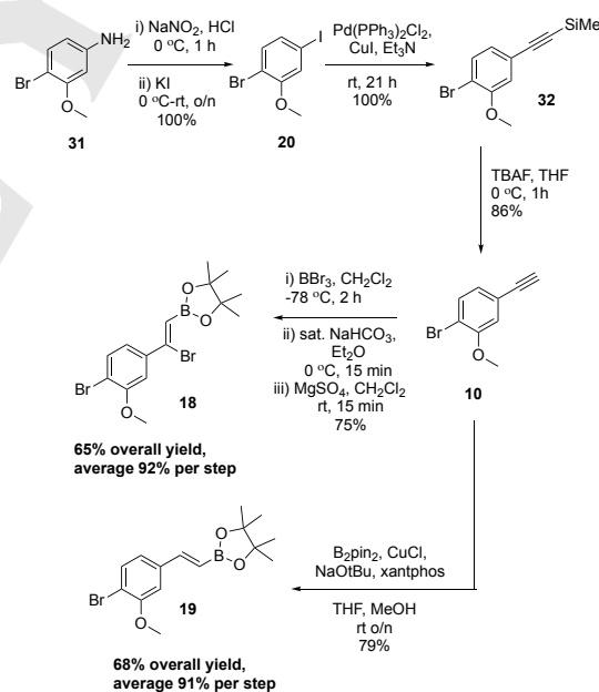
Scheme 5. Current route to key aryl intermediates 10 , 18 and 19 .
