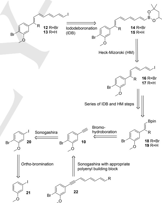
Scheme 2. Retrosynthesis of either tetraene 12 or 13 and alkynyl polyene 22 .
