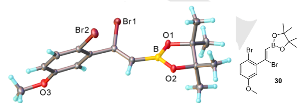
Figure 2. X-ray molecular structure of boronate ester 30 [CCDC-1537382]; thermal ellipsoids shown at 50% probability].
