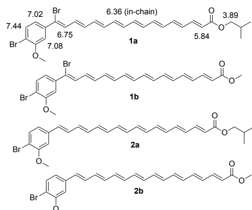
Figure 1. Structures of the various xanthomonadin analogues and ^1\text{H} NMR data as reported by Andrewes et al. for isobutyl xanthomonadin 1a . [24]
