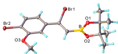
Figure 3. X-ray molecular structure of boronate ester 18 (CCDC-1537383).
