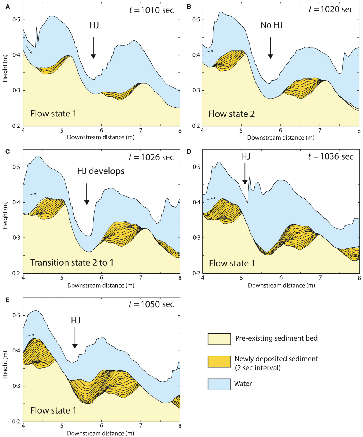
Fig. 7. Five panels showing the flow behaviour during different stages of the cyclic step system, also shown are the associated newly formed deposits. The lines in the newly formed deposits are two-second timelines.
