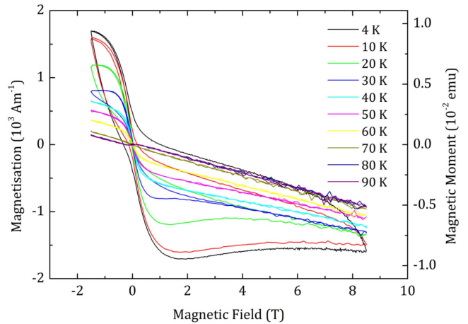
Figure 14. Magnetisation as a function of field the B1M30HA750 sample between -1.5 and 8 T at temperatures between 4 and 90 K. The data at -1.5 T have a gradient \mu_0 \Delta M / \Delta B of -3 \times 10^{-3} .
