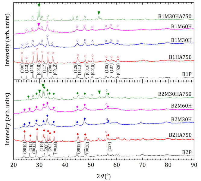
Figure 2. XRD of B1 (upper panel) and B2 (lower panel) samples. From the bottom to the top, the traces in each panel are: as-supplied material, HA750, M30H, M60H and M30HA750 samples. The main \text{Bi}_2\text{Sr}_2\text{CuO}_6 , \text{Bi}_2\text{Sr}_2\text{CaCu}_2\text{O}_8 and \text{Bi}_2\text{Sr}_2\text{Ca}_2\text{Cu}_3\text{O}_{10} peaks are labelled with ‘▼’, ‘○’ and ‘◆’ symbols respectively.
