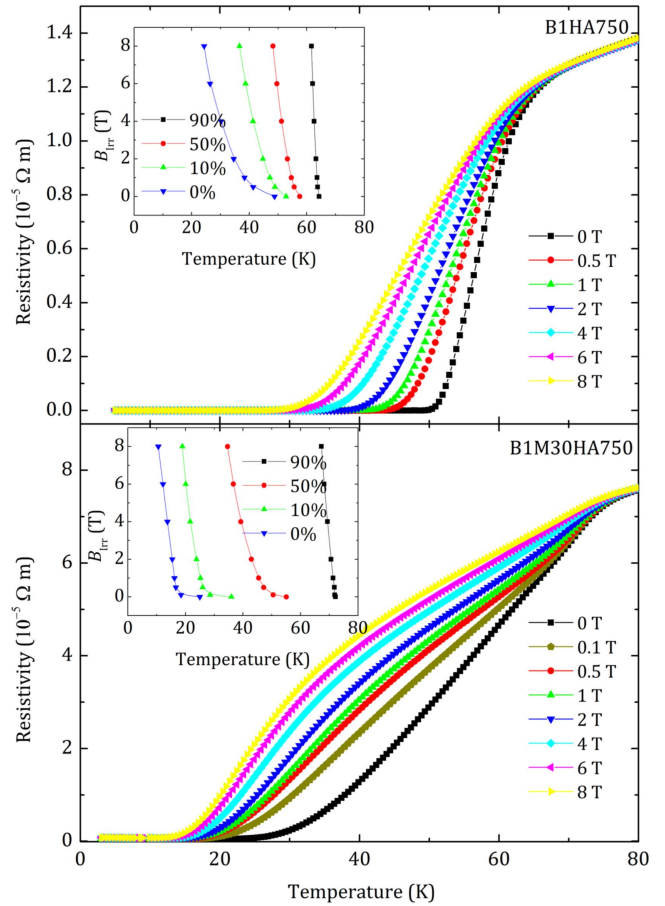
Figure 6. Upper panel: resistivity of the B1HA750 sample measured in fields of 0–8 T with a constant excitation current of 5 mA. Inset: B_{\text{irr}} determined using the criteria of 90%, 50% and 10% of \rho_N(0\text{ T}, 70\text{ K}) , and onset of zero resistivity (0% \rho_N ). Lower panel: equivalent data for the B1M30HA750 sample.
