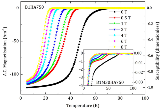
Figure 9. Ac magnetic susceptibility as a function of temperature of the B1HA750 sample. The data were taken with an excitation field of 0.4 mT and at a frequency of 777 Hz. Inset: equivalent data for the B1M30HA750 sample.
