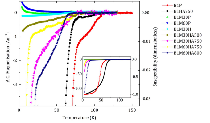
Figure 8. A.C. magnetisation and magnetic susceptibility of all B1 samples in zero field. The data were taken with an excitation field of 0.4 mT at a frequency of 777 Hz. Inset: equivalent large signal data.
