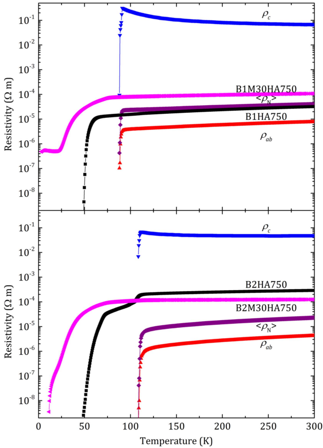
Figure 5. Resistivity as a function of temperature for \text{Bi}_2\text{Sr}_2\text{CaCu}_2\text{O}_8 (upper panel) and \text{Bi}_2\text{Sr}_2\text{Ca}_2\text{Cu}_3\text{O}_{10} (lower panel) micro-(HA750) and nanocrystalline (M30HA750) materials in zero field.
