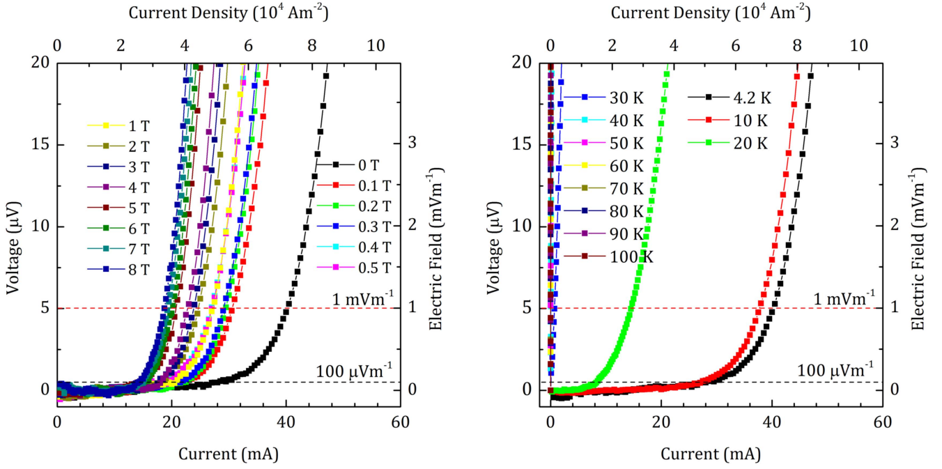
Figure 21. Left: voltage as a function of current for the B1M30HA750 sample at 4.2 K. The dashed lines show the field criteria of 1 \text{ mVm}^{-1} and 100 \text{ } \mu\text{Vm}^{-1} . Right: voltage as a function of current at different temperatures in zero field.
