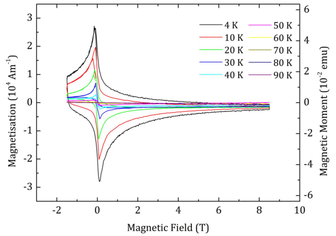
Figure 13. Magnetisation as a function of field of the B1HA750 sample between -1.5 and 8 T at temperatures between 4 and 90 K. The data at -1.5 T have a gradient \mu_0 \Delta M / \Delta B of -0.2 .
