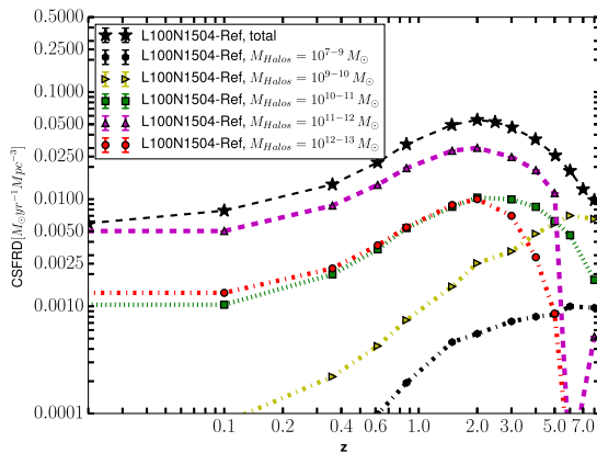
Figure 4. CSFRD contribution of haloes with different masses in EAGLE. Below redshift 5 objects with masses M_{\text{halo}} = 10^{11-12} M_\odot dominate through their high efficiencies besides their low numbers (Fig. 5).
