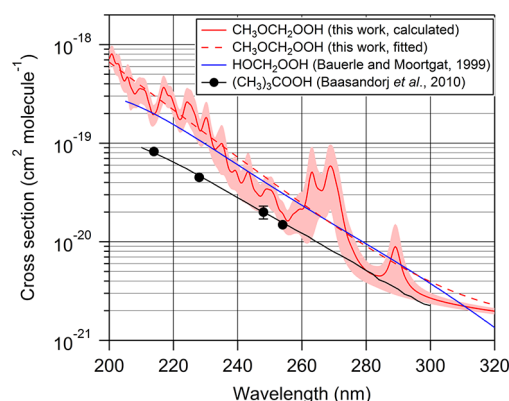
Figure 5. Calculated UV absorption cross-section for the simplest \alpha -alkoxyalkyl hydroperoxide (AAAH), methoxymethyl hydroperoxide (MMHP). A close similarity is observed between MMHP and the literature measurement for hydroxymethyl hydroperoxide, suggesting a commonality in the photochemistry of AAAHs.
