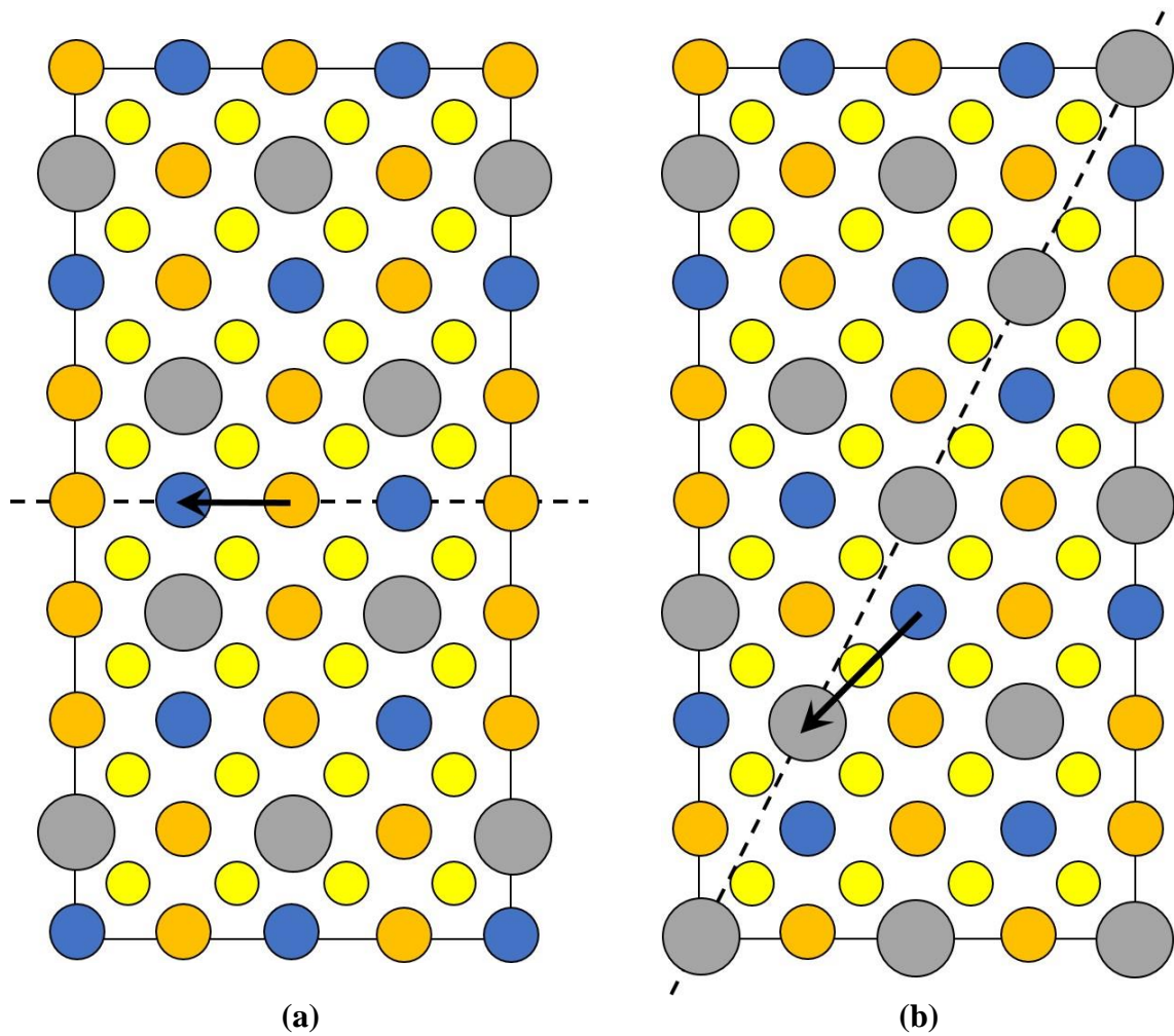
Figure 2: Supercell of the (a) \frac{1}{2}[110] (001) and (b) \frac{1}{4}[201] (101) ASBs in kesterite viewed along [100] (the vertical axis is [001], while the horizontal axis is [010]). Cu, Zn, Sn and Se atoms are depicted by orange, blue, silver and yellow circles respectively. The dashed line represents the ASB plane and the arrow the ASB shear vector projected onto the [100] viewing plane. In both figures the bottom half of the crystal is displaced with respect to the top half. Figures adapted from reference [15].
